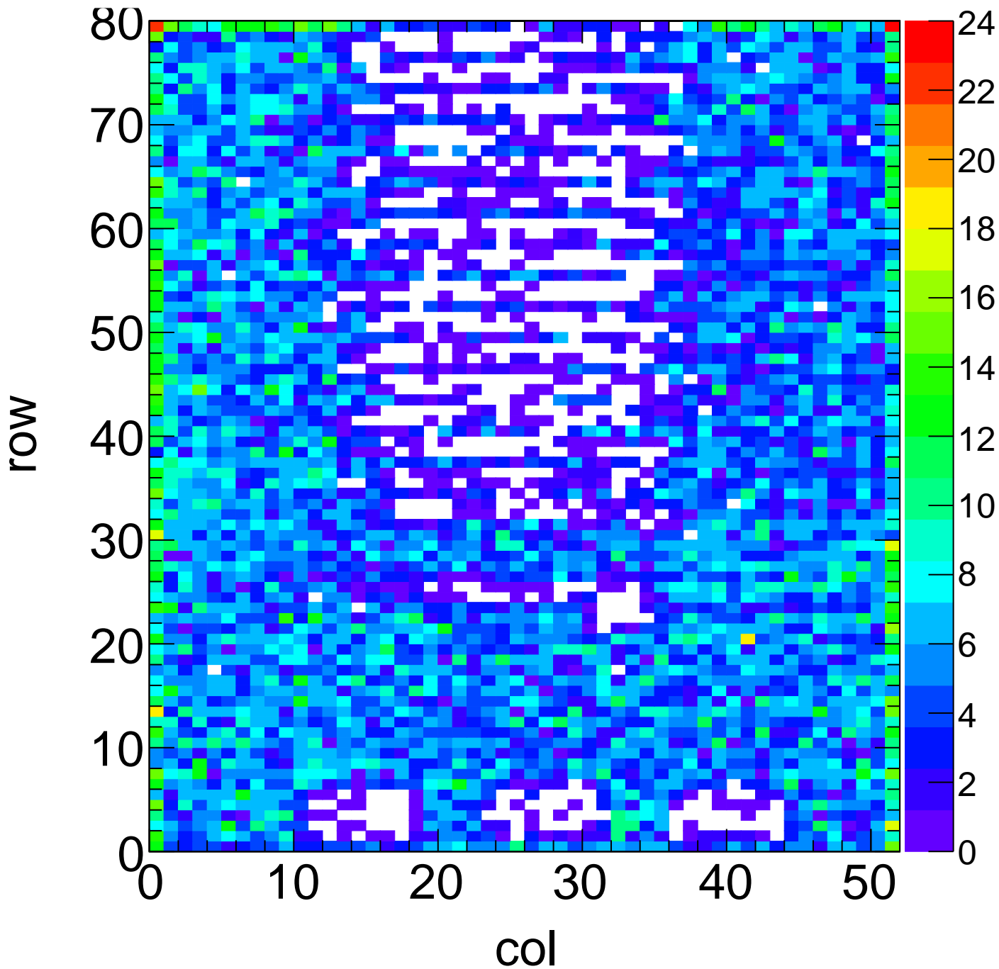
X-ray Hit Map - Target Ag Method Spectrum Chip C13
