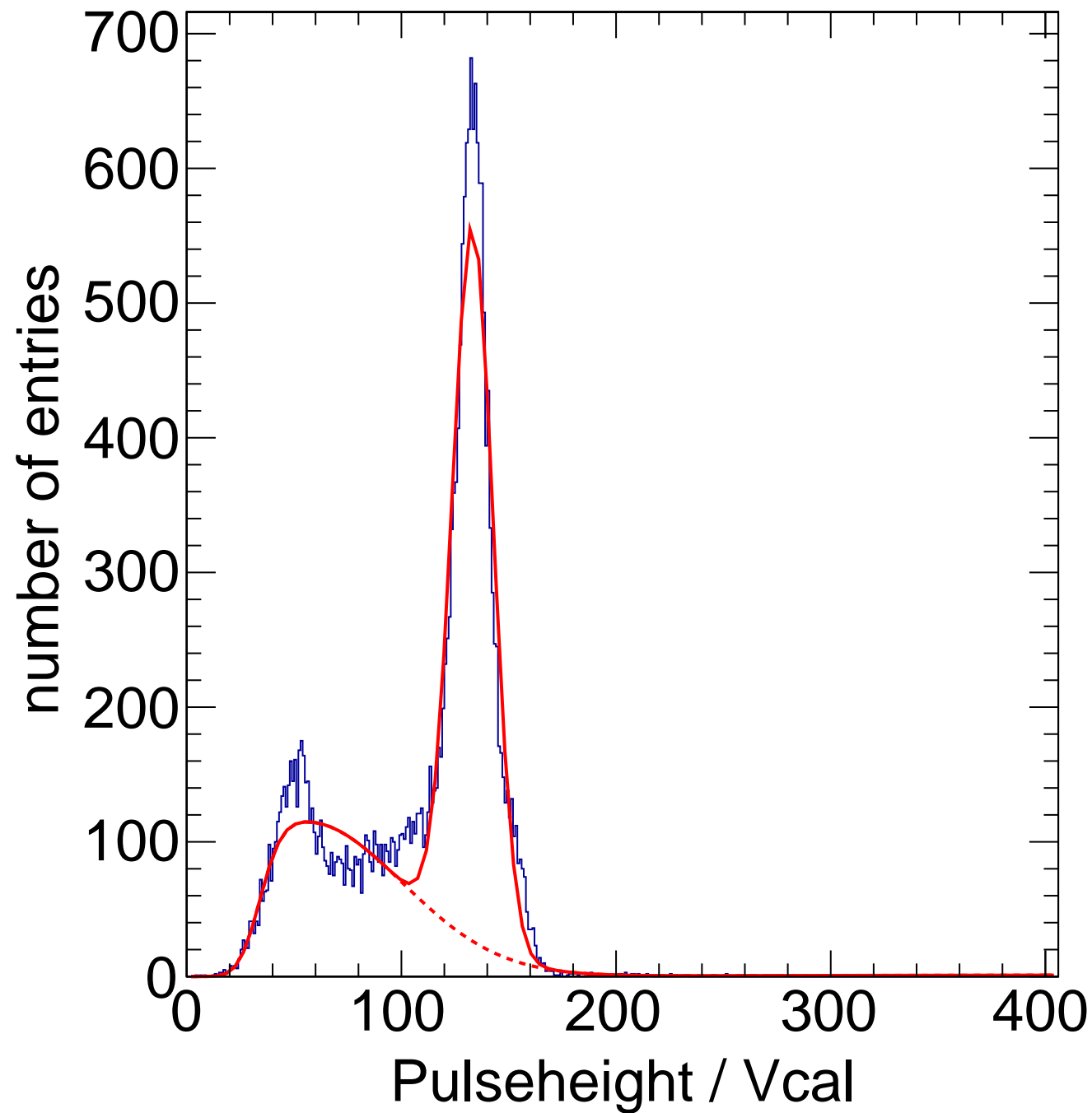
X-ray Calibration - Target Ag Method Spectrum Chip C8
