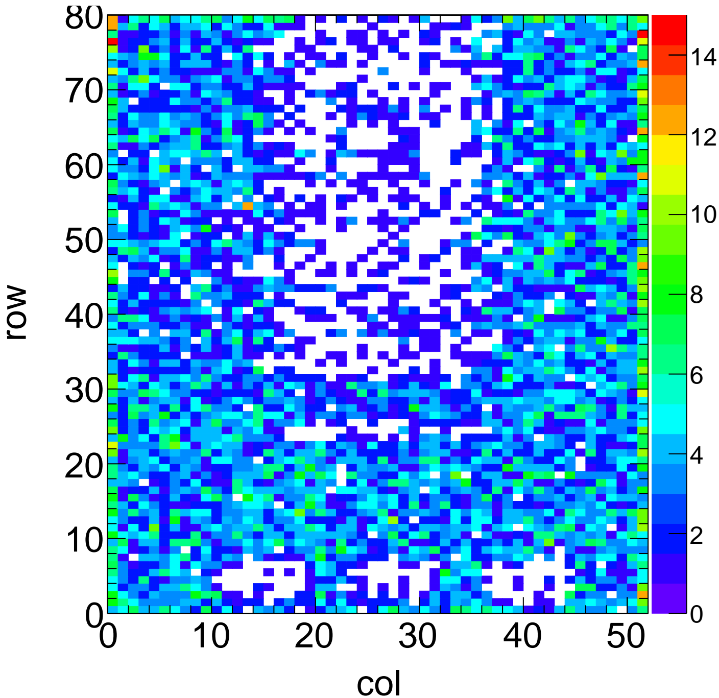
X-ray Hit Map - Target Sn Method Spectrum Chip C2
