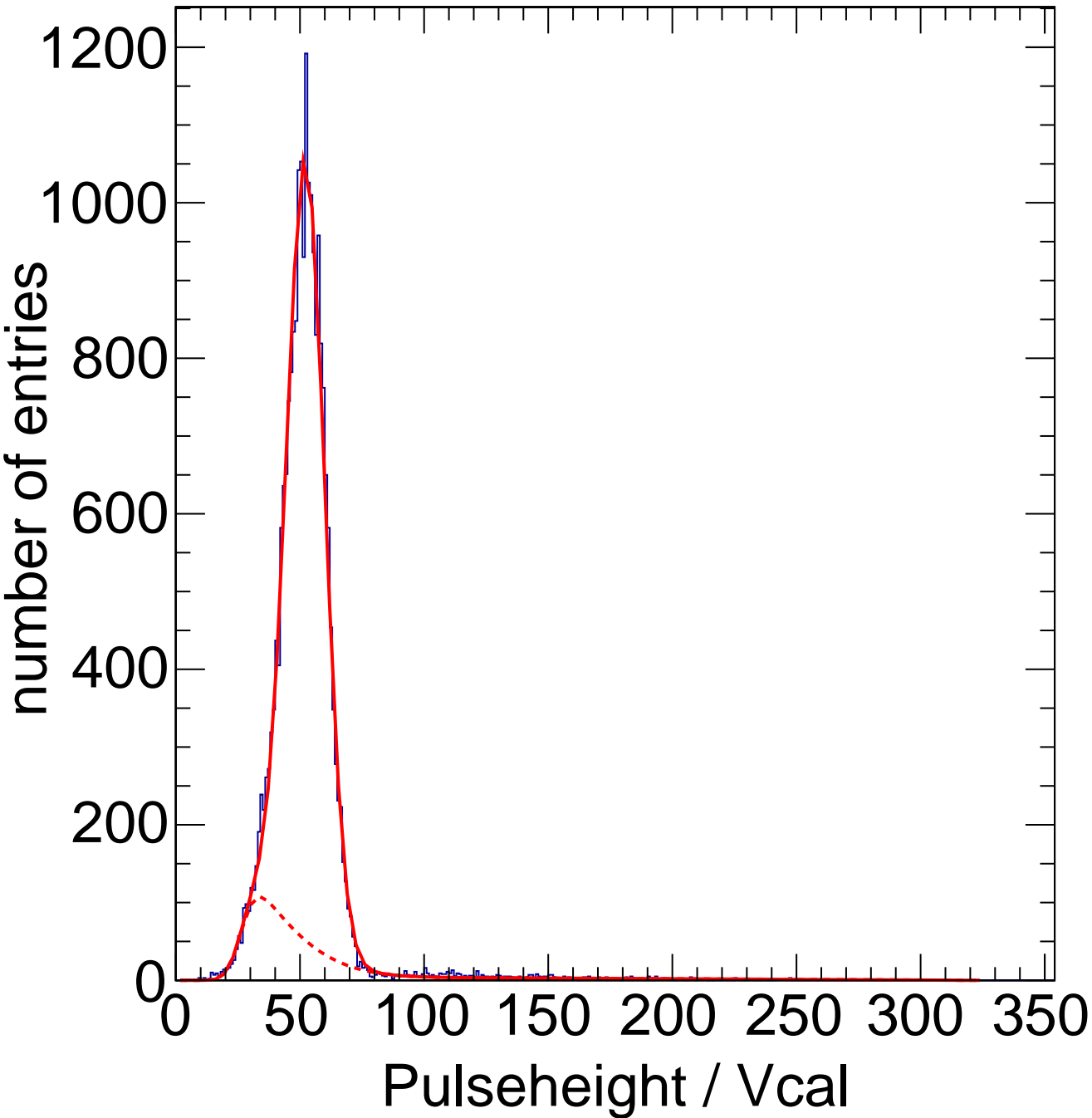
X-ray Calibration - Target Zn Method Spectrum Chip C3
