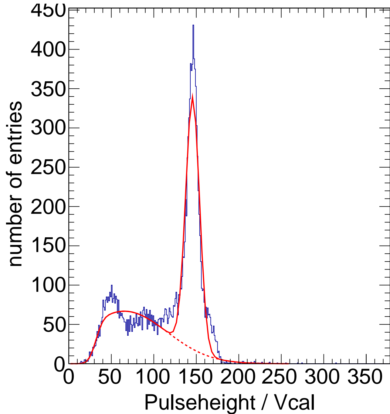
X-ray Calibration - Target Sn Method Spectrum Chip C4
