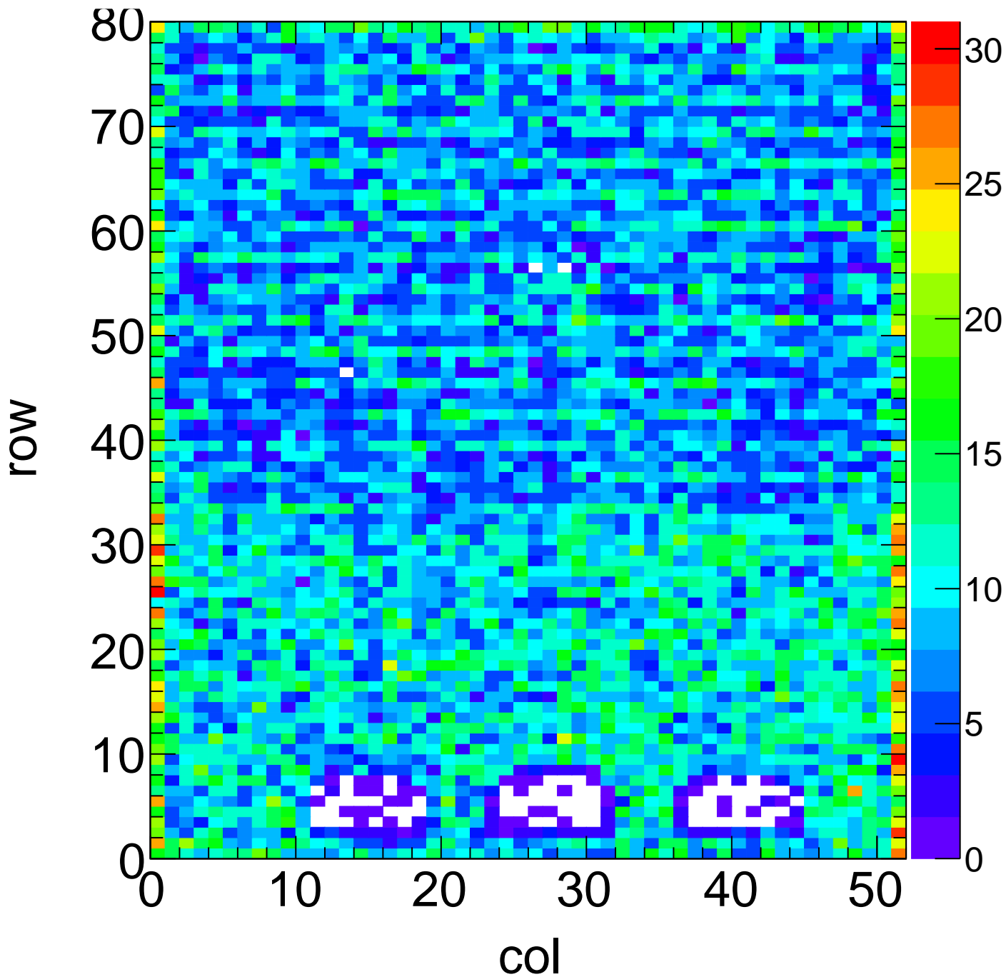
X-ray Hit Map - Target Mo Method Spectrum Chip C15
