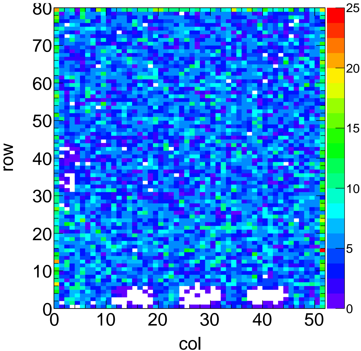
X-ray Hit Map - Target Ag Method Spectrum Chip C0
