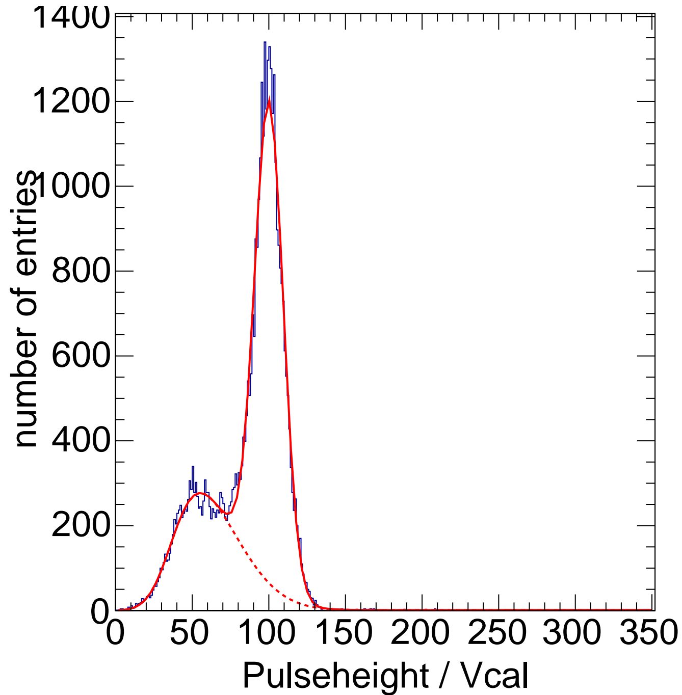
X-ray Calibration - Target Mo Method Spectrum Chip C3
