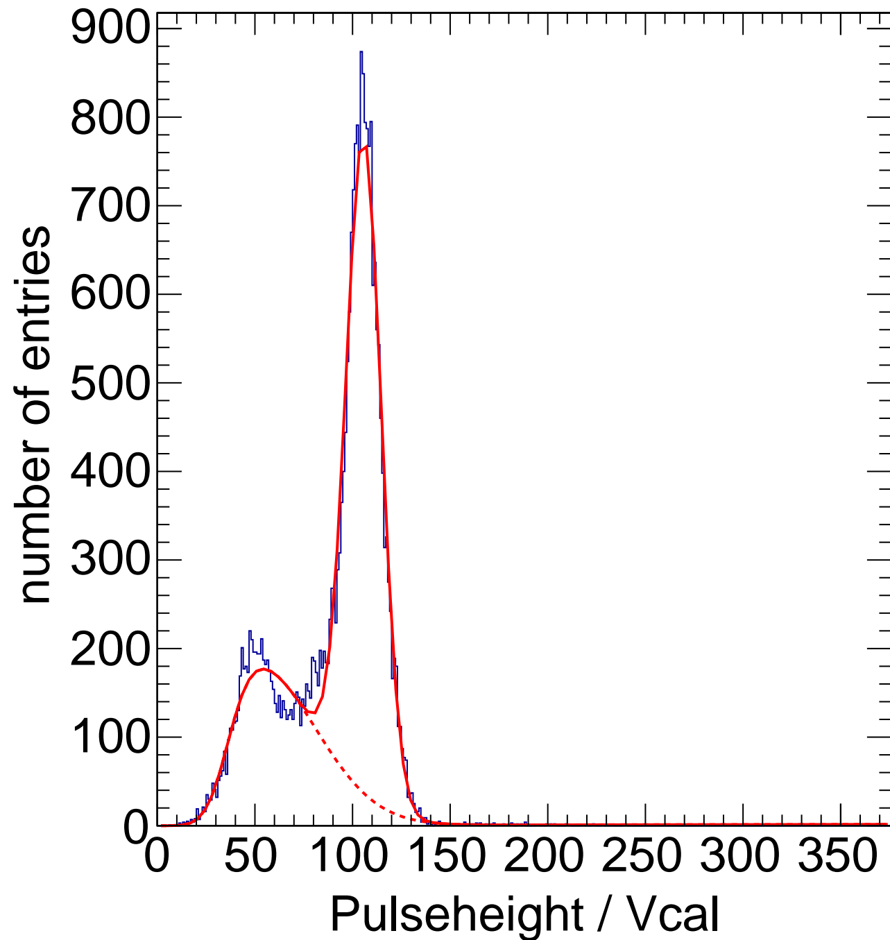
X-ray Calibration - Target Mo Method Spectrum Chip C13
