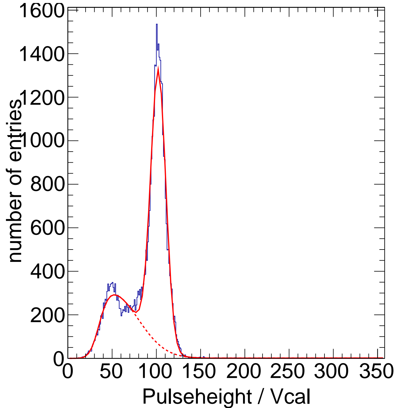
X-ray Calibration - Target Mo Method Spectrum Chip C8
