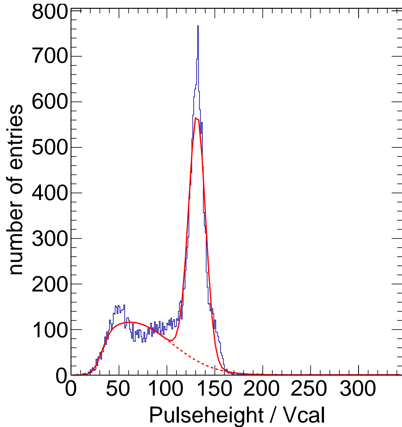
X-ray Calibration - Target Ag Method Spectrum Chip C6
