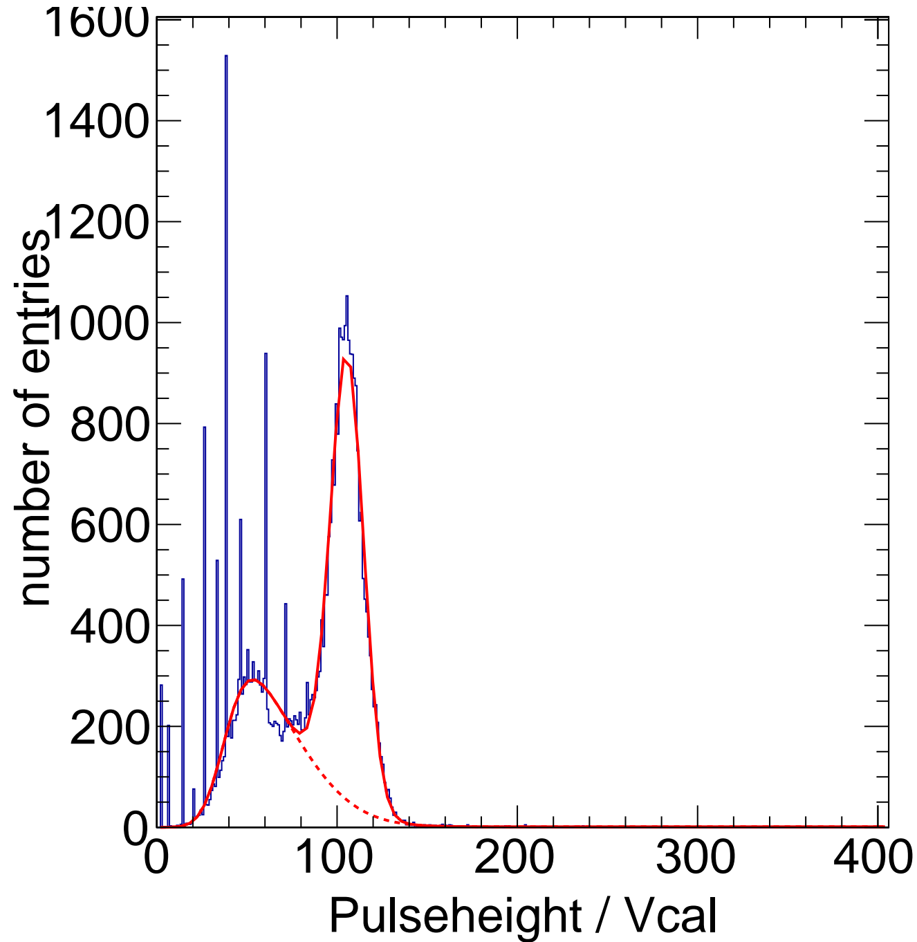
X-ray Calibration - Target Mo Method Spectrum Chip C0
