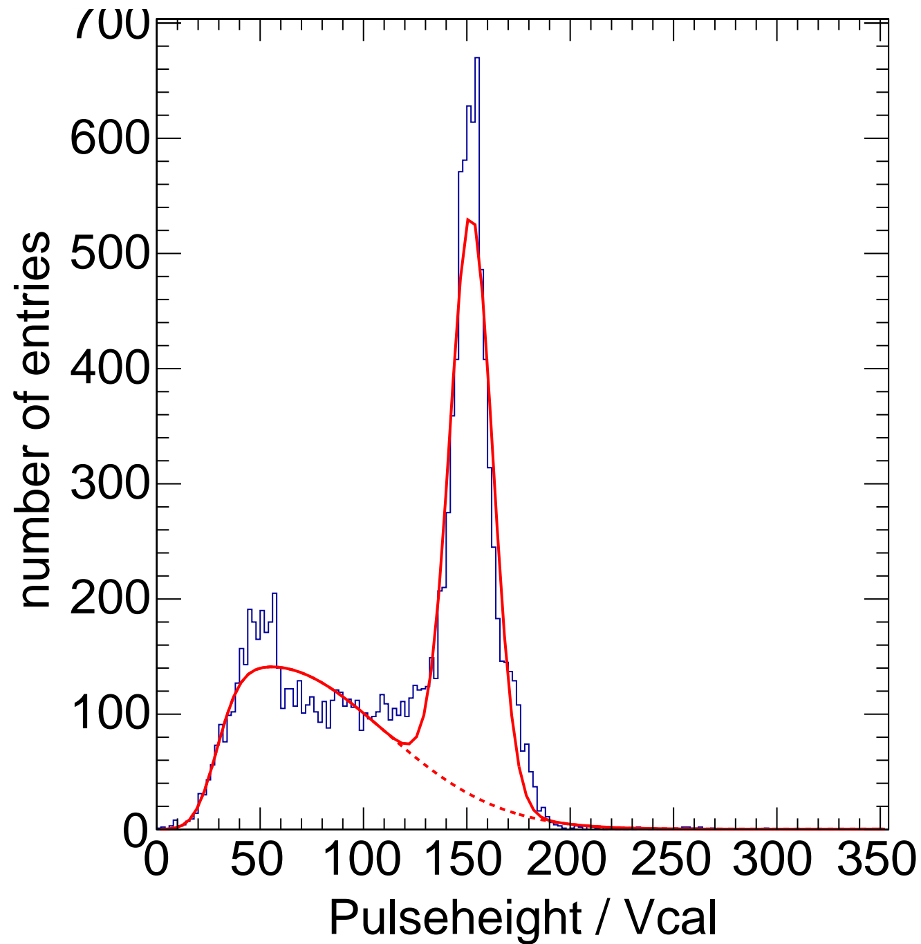
X-ray Calibration - Target Sn Method Spectrum Chip C8
