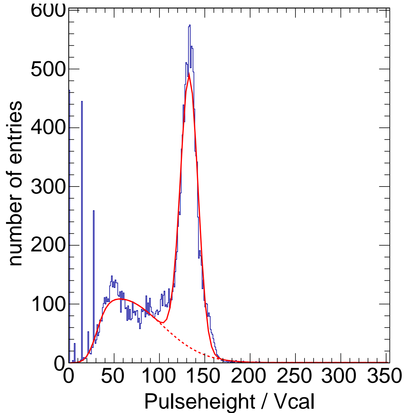
X-ray Calibration - Target Ag Method Spectrum Chip C4
