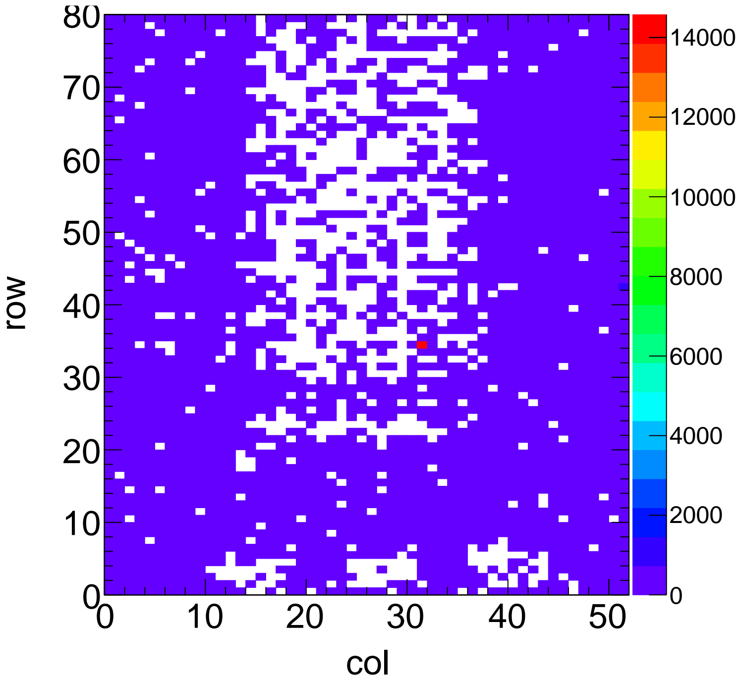
X-ray Hit Map - Target Sn Method Spectrum Chip C2
