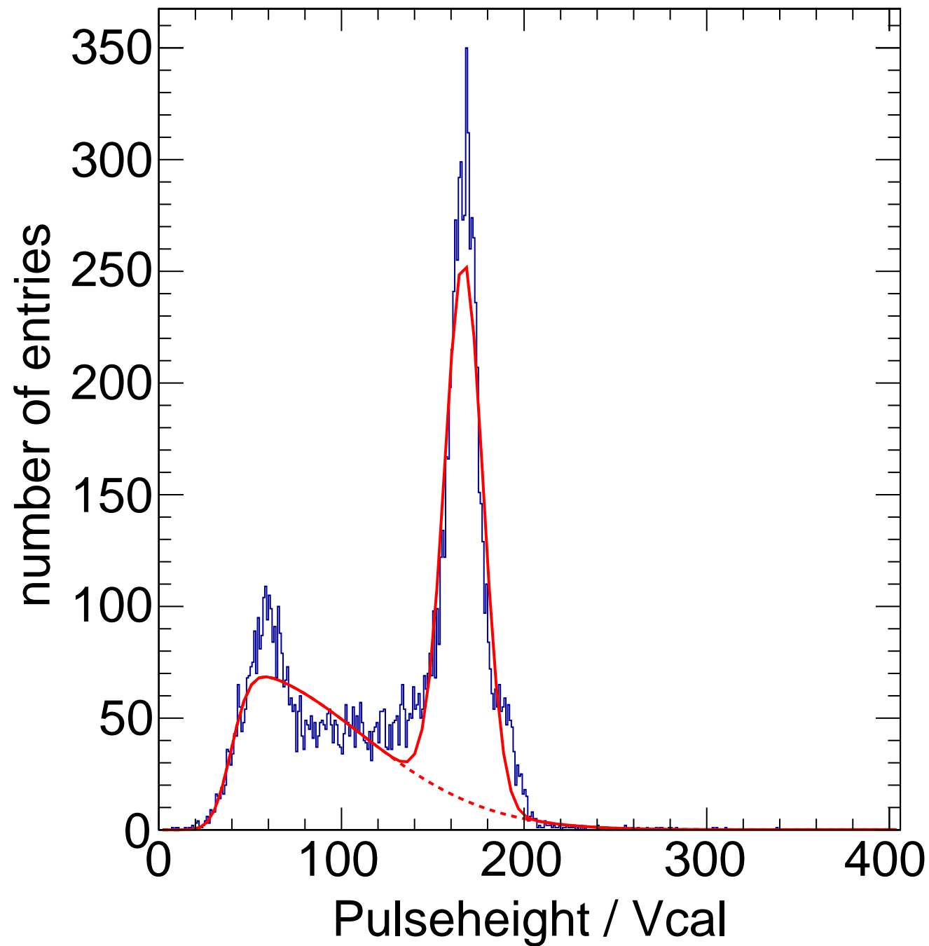
X-ray Calibration - Target Sn Method Spectrum Chip C14
