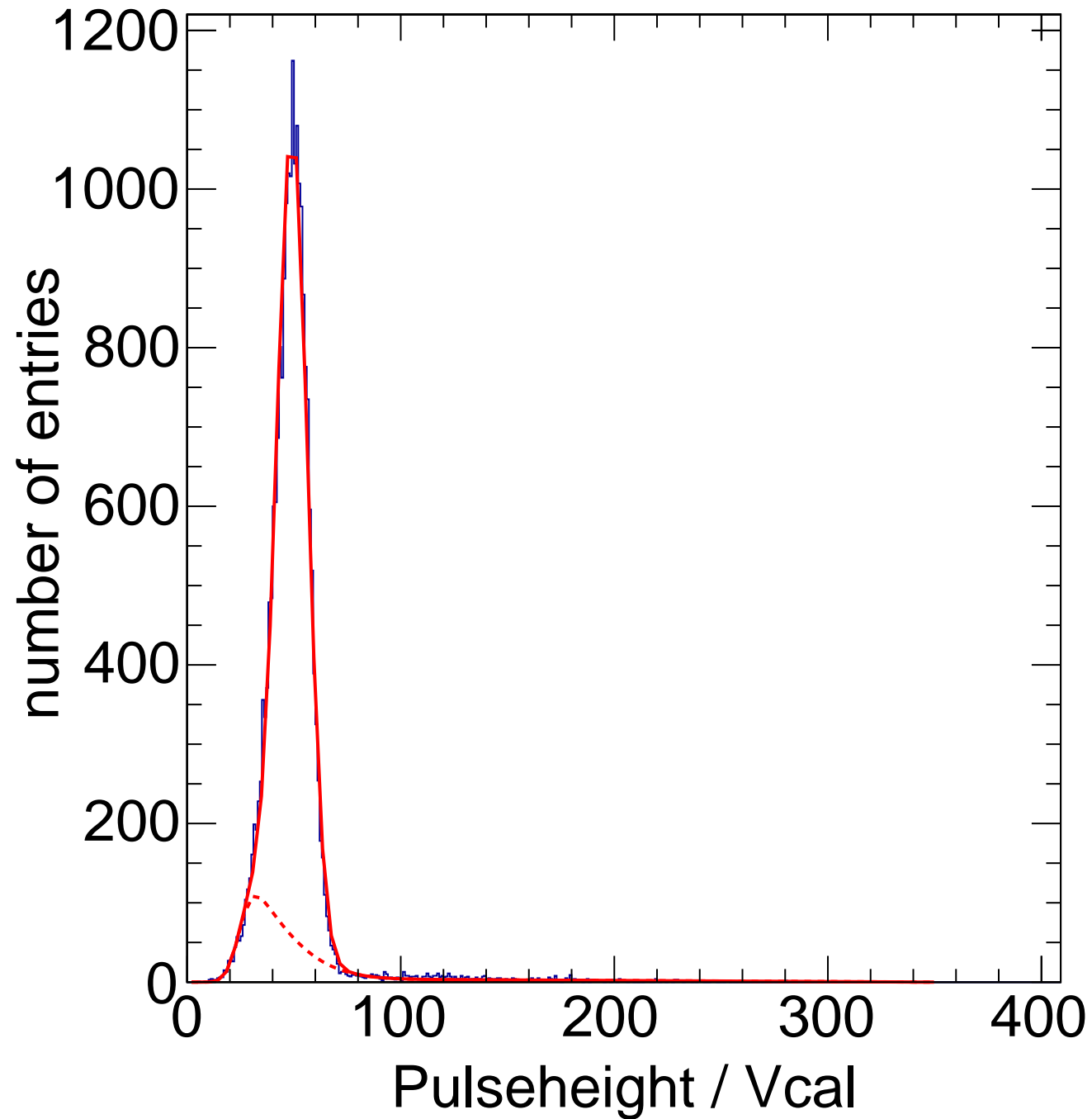
X-ray Calibration - Target Zn Method Spectrum Chip C14
