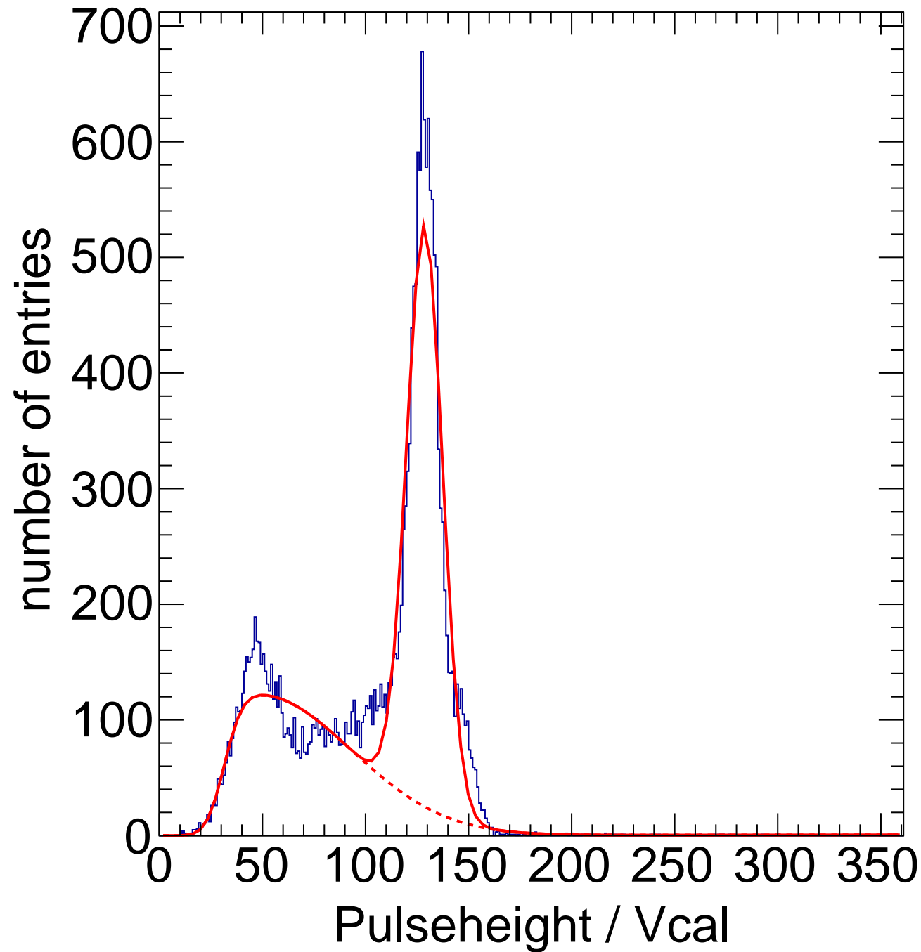
X-ray Calibration - Target Ag Method Spectrum Chip C14
