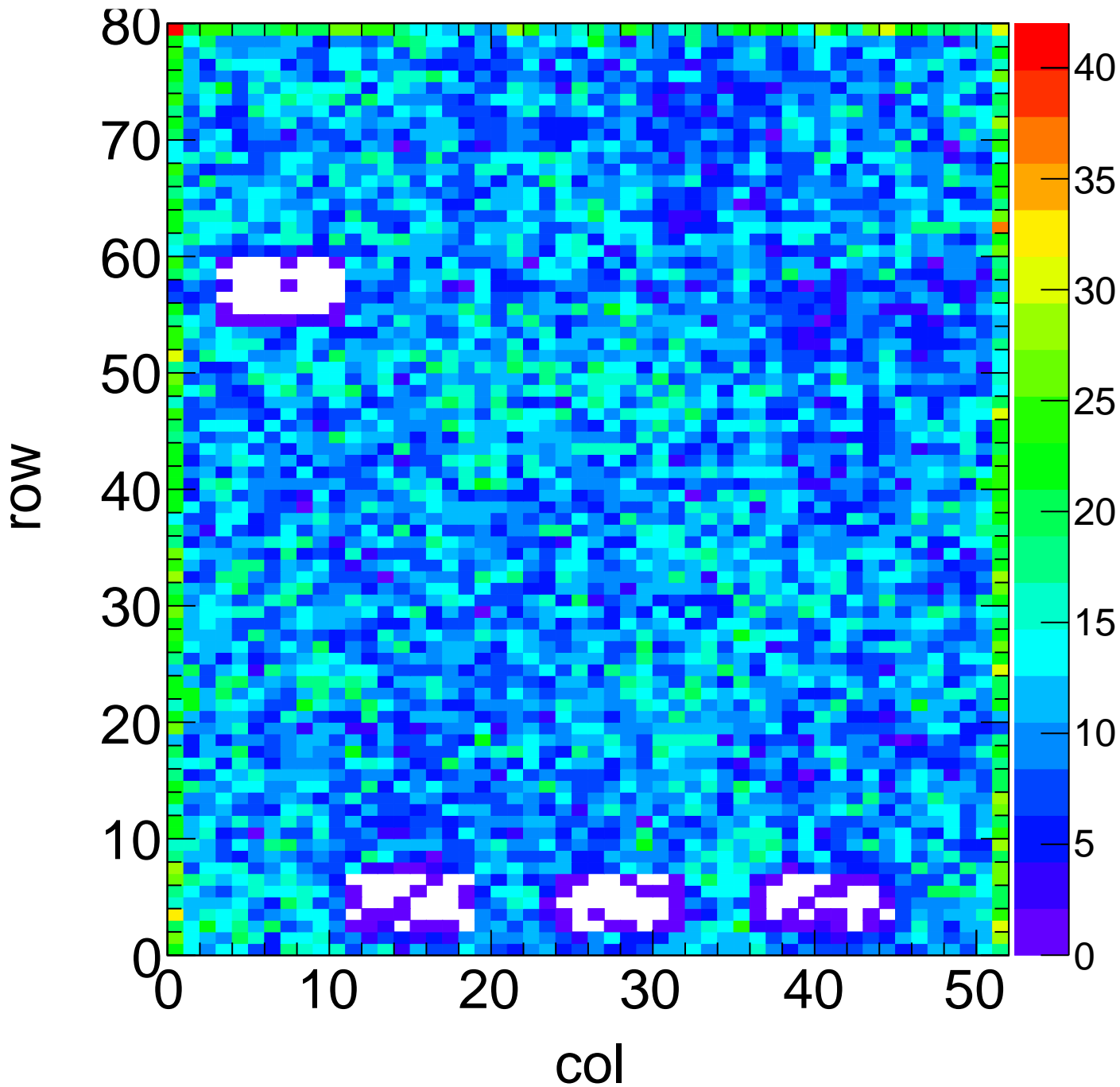
X-ray Hit Map - Target Mo Method Spectrum Chip C11
