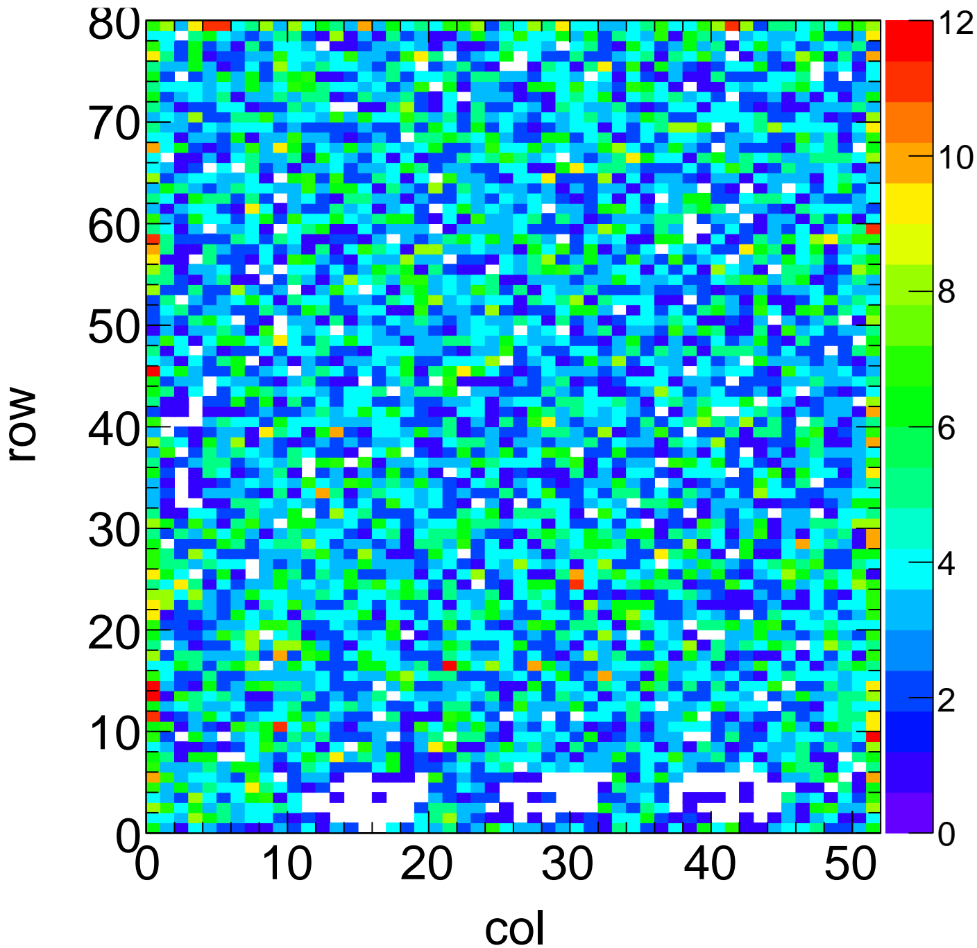
X-ray Hit Map - Target Sn Method Spectrum Chip C0
