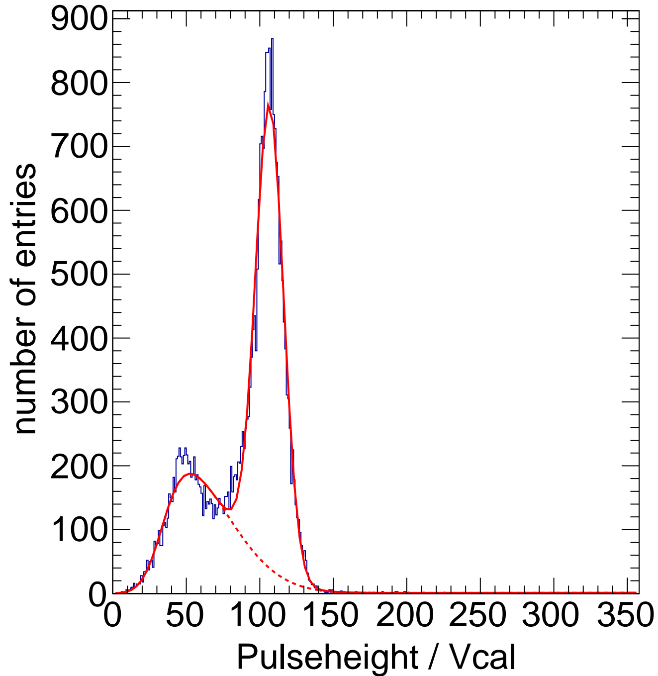
X-ray Calibration - Target Mo Method Spectrum Chip C2
