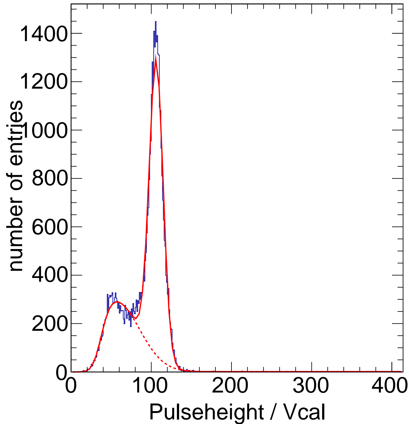
X-ray Calibration - Target Mo Method Spectrum Chip C12
