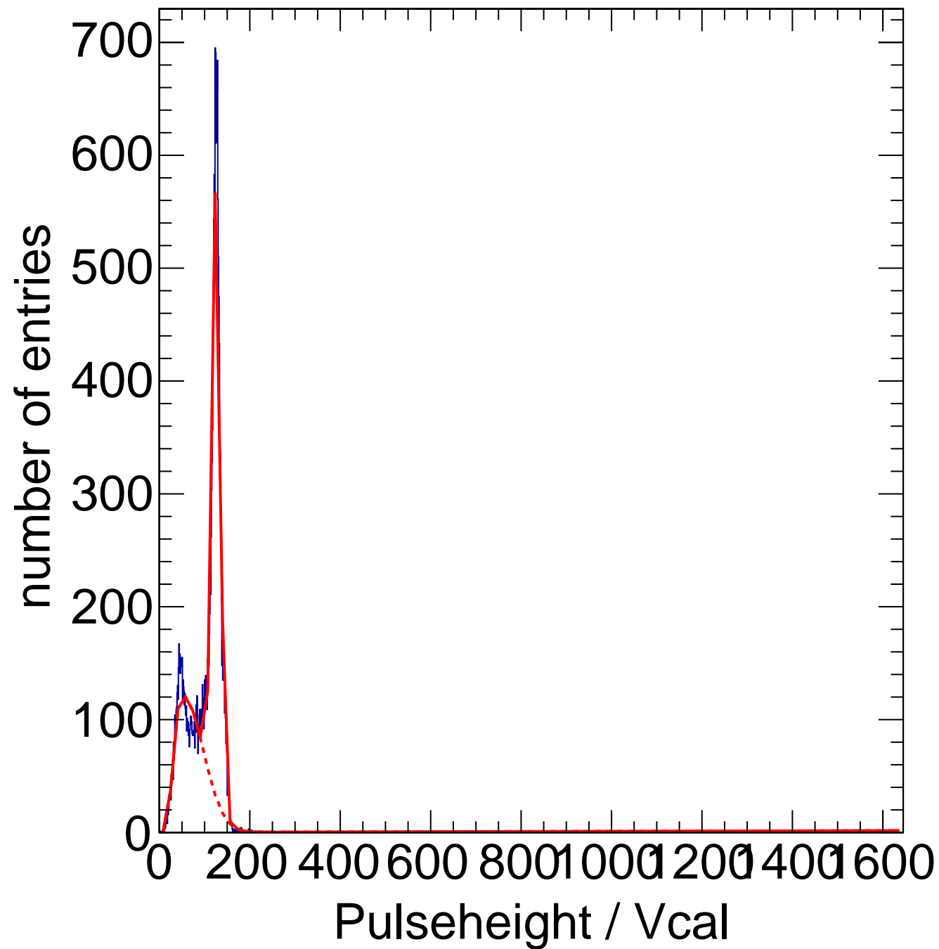
X-ray Calibration - Target Ag Method Spectrum Chip C12
