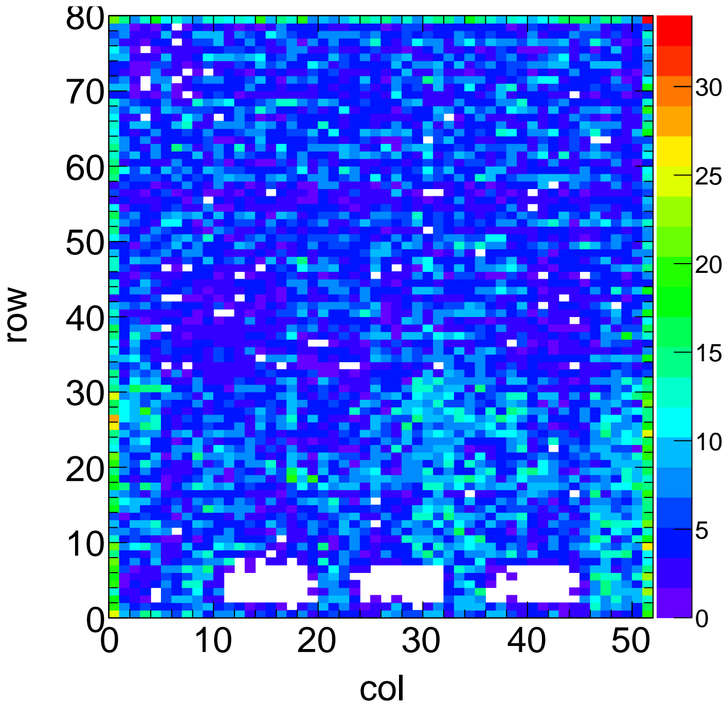
X-ray Hit Map - Target Zn Method Spectrum Chip C15
