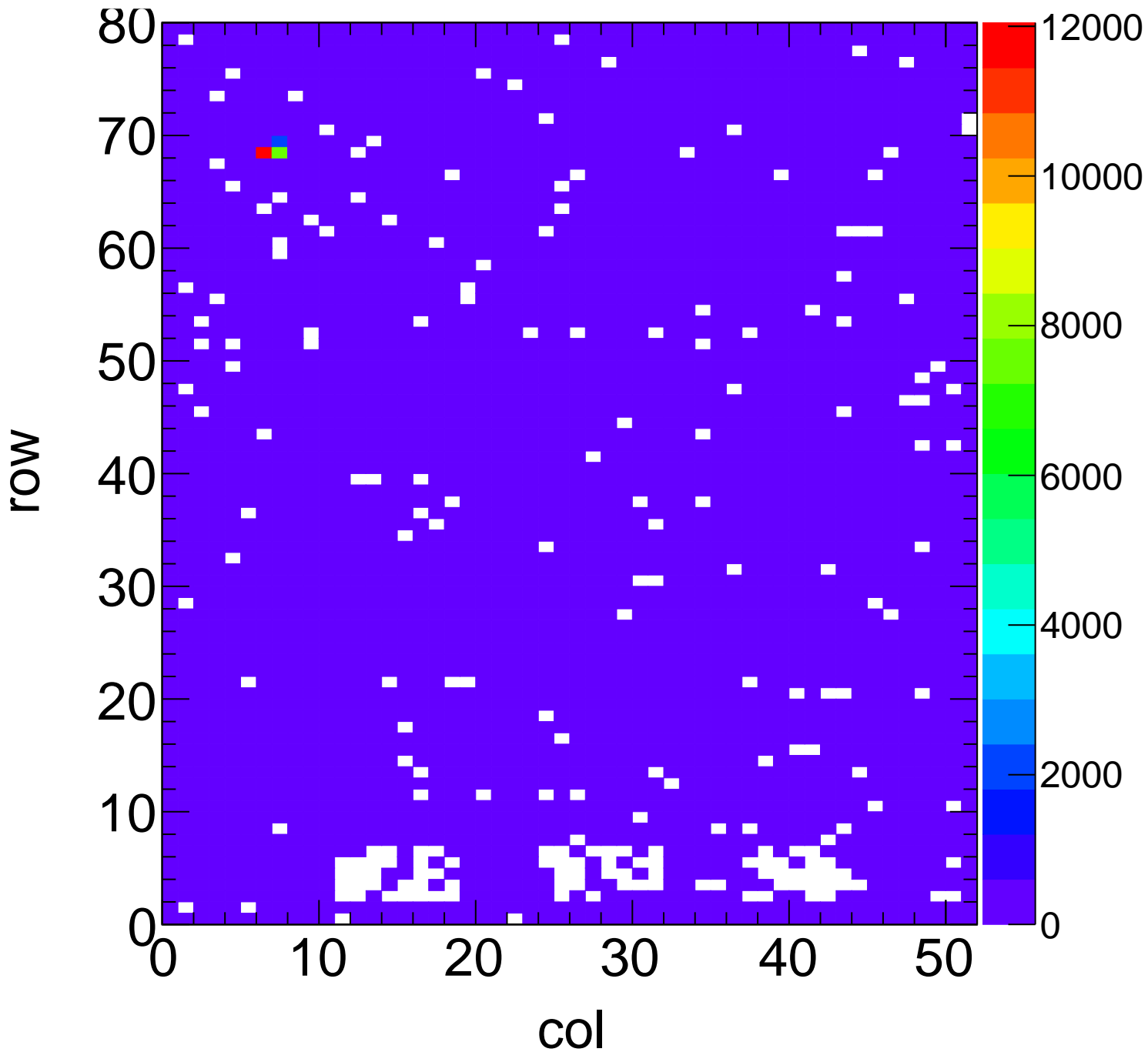
X-ray Hit Map - Target Sn Method Spectrum Chip C12
