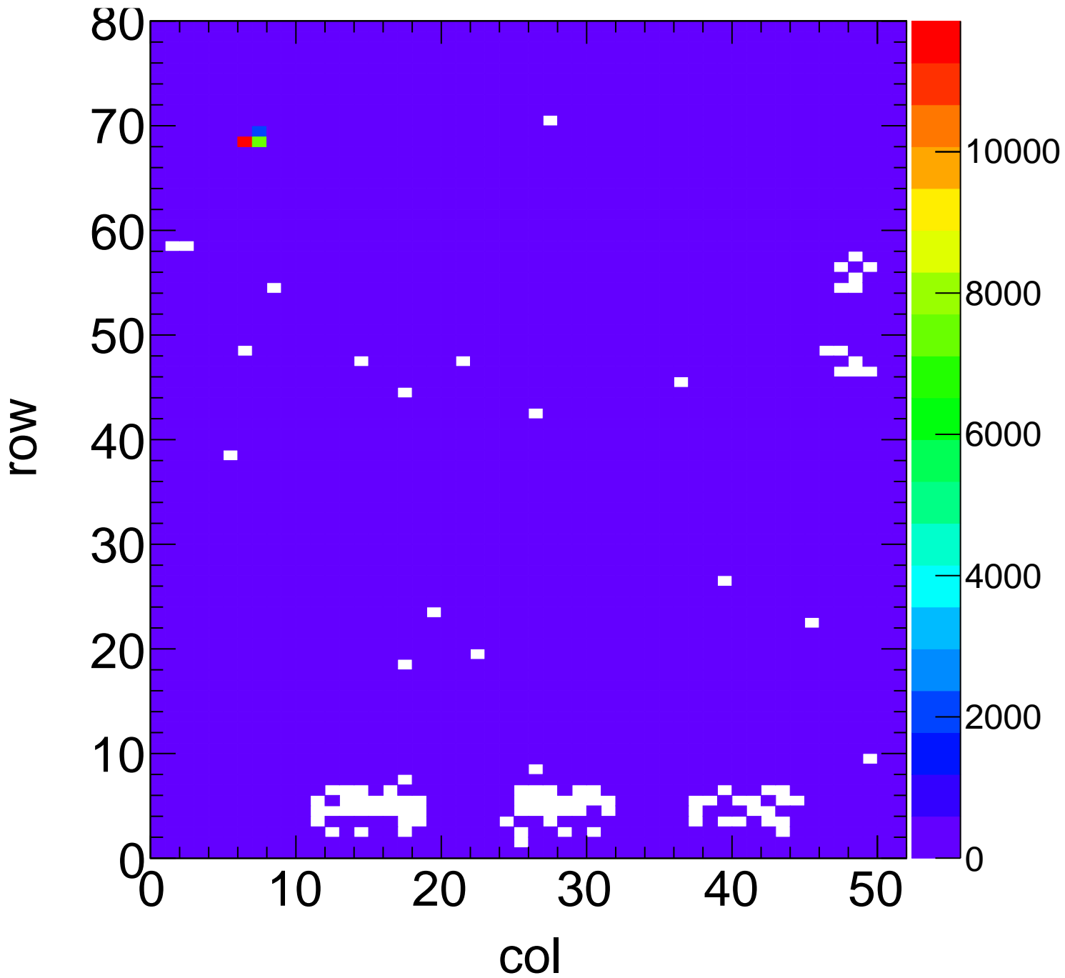
X-ray Hit Map - Target Ag Method Spectrum Chip C12
