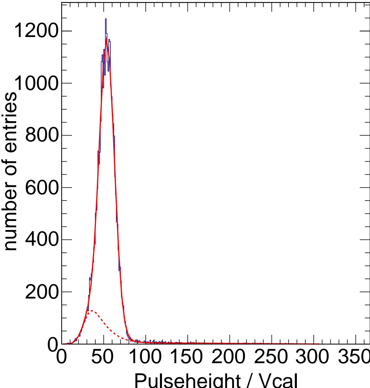
X-ray Calibration - Target Zn Method Spectrum Chip C6
