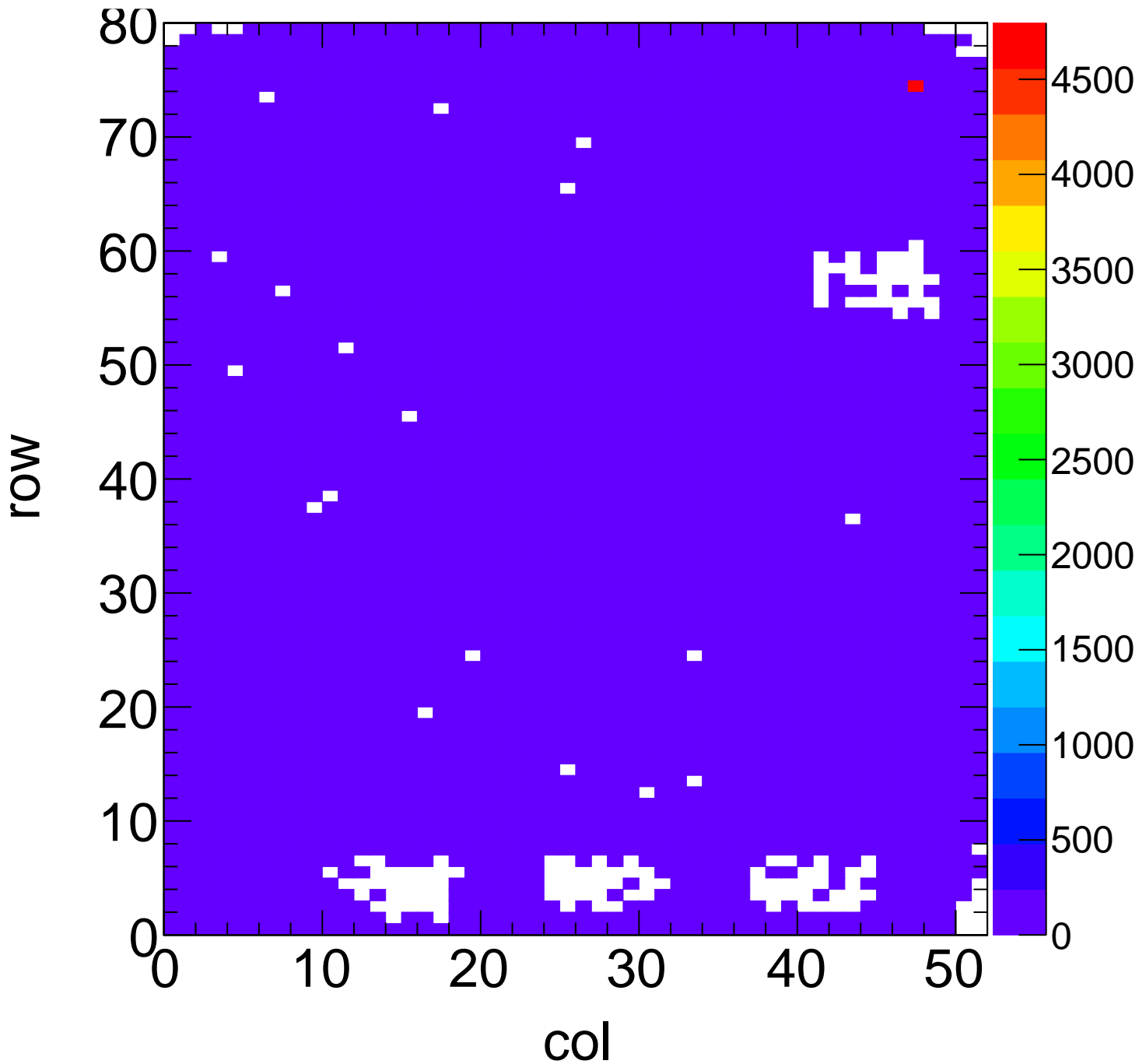
X-ray Hit Map - Target Ag Method Spectrum Chip C4
