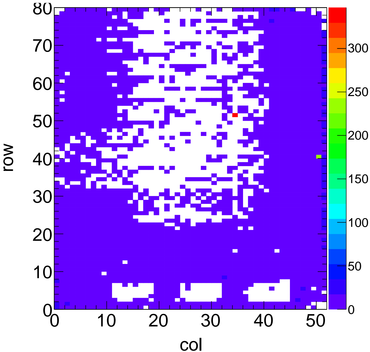
X-ray Hit Map - Target Zn Method Spectrum Chip C2
