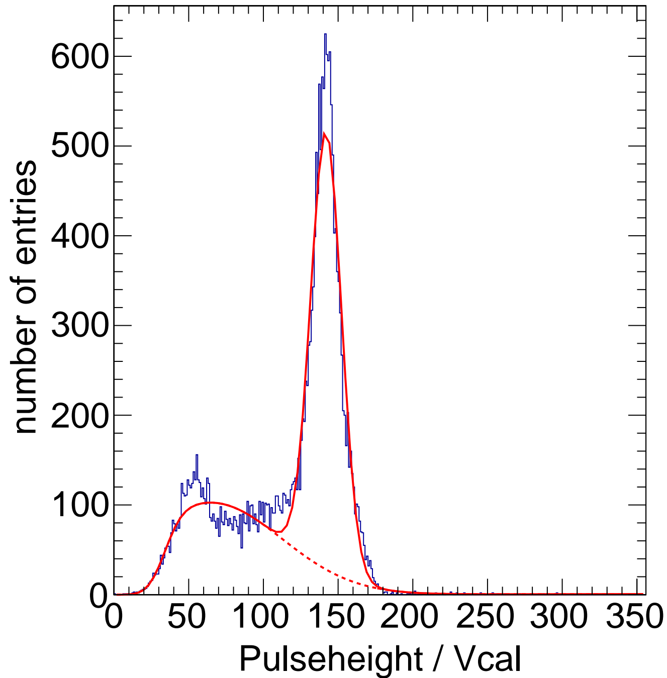
X-ray Calibration - Target Ag Method Spectrum Chip C11
