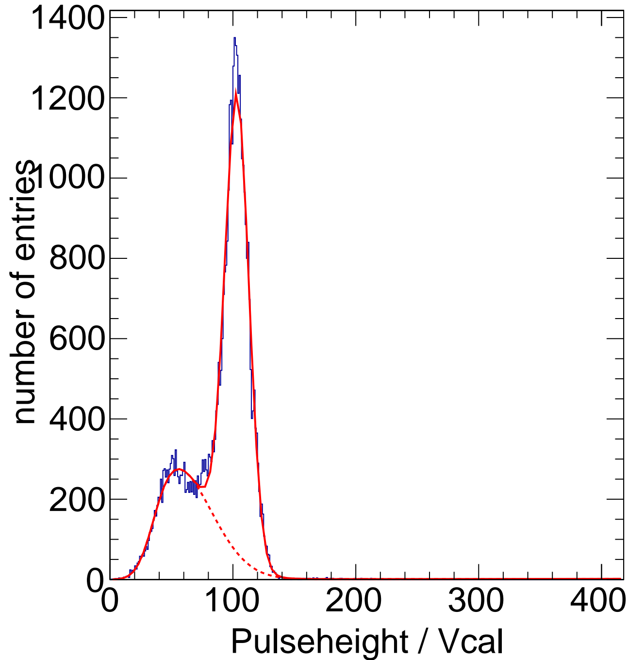
X-ray Calibration - Target Mo Method Spectrum Chip C7
