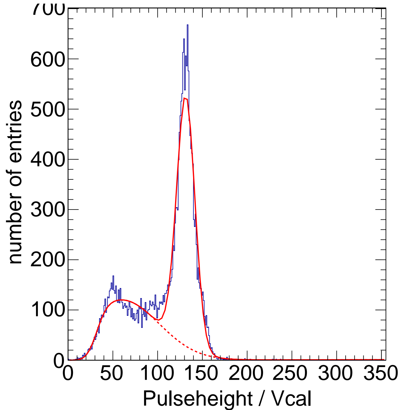
X-ray Calibration - Target Ag Method Spectrum Chip C7
