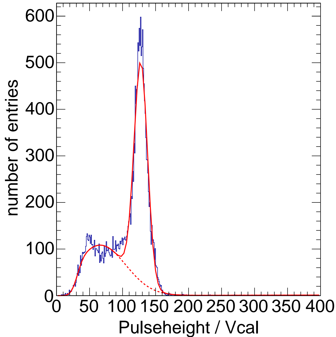
X-ray Calibration - Target Ag Method Spectrum Chip C3
