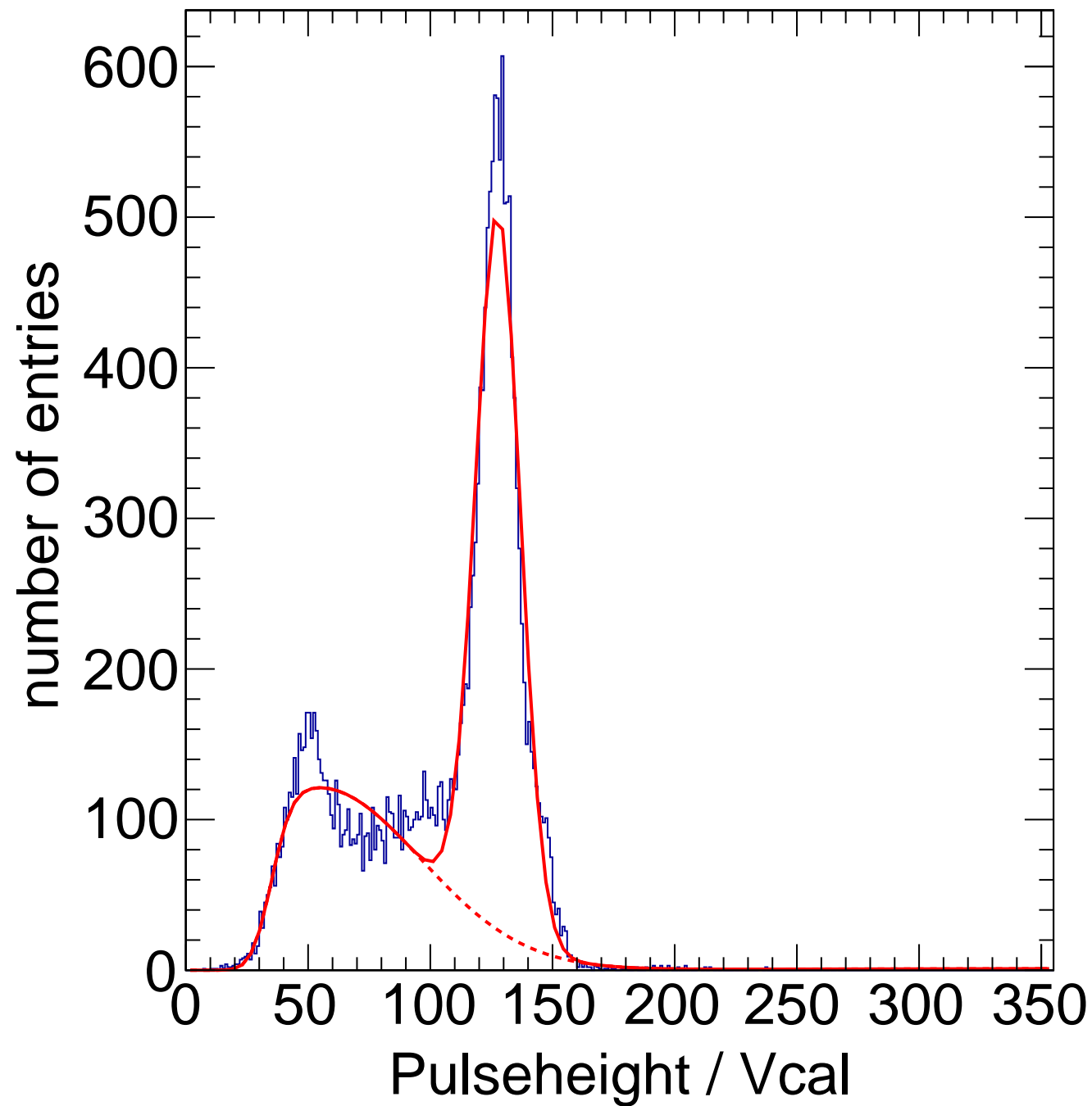
X-ray Calibration - Target Ag Method Spectrum Chip C14
