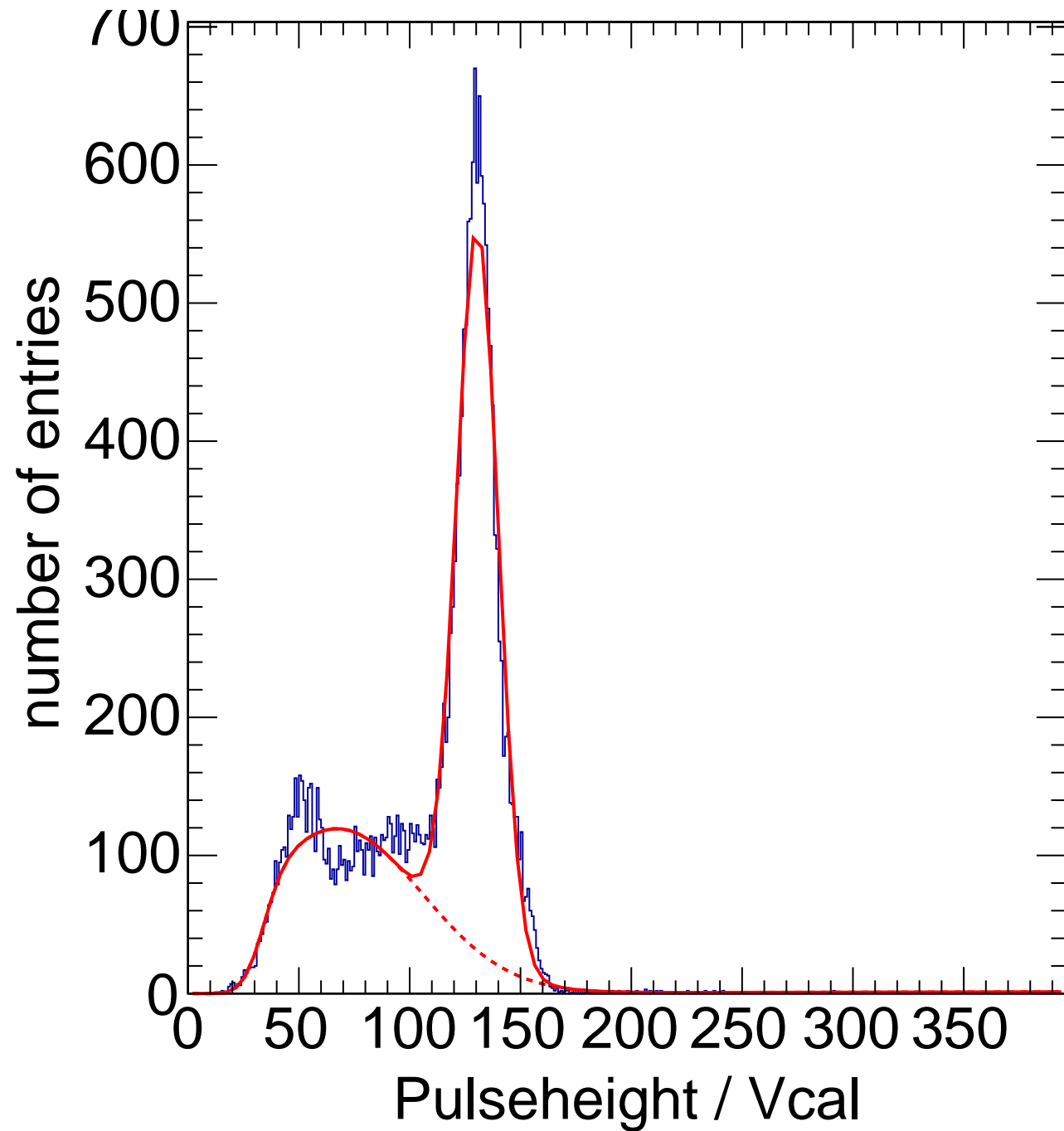
X-ray Calibration - Target Ag Method Spectrum Chip C11
