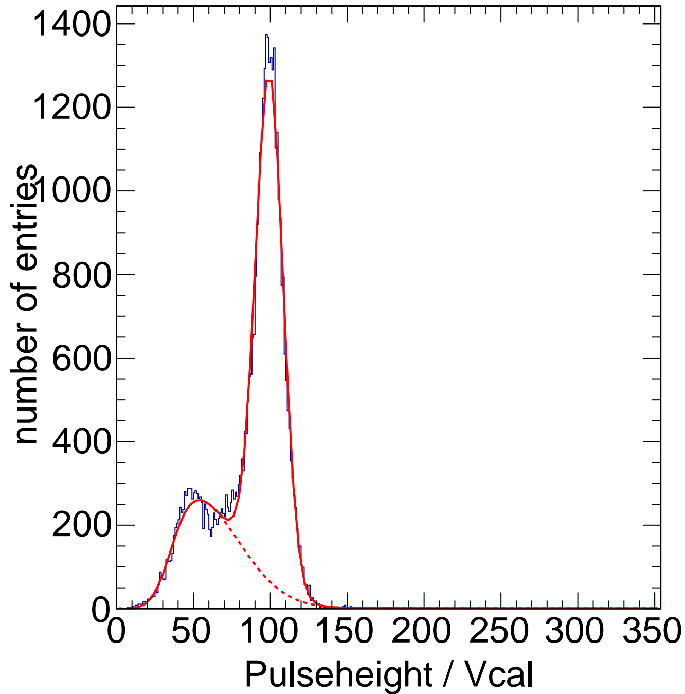
X-ray Calibration - Target Mo Method Spectrum Chip C4
