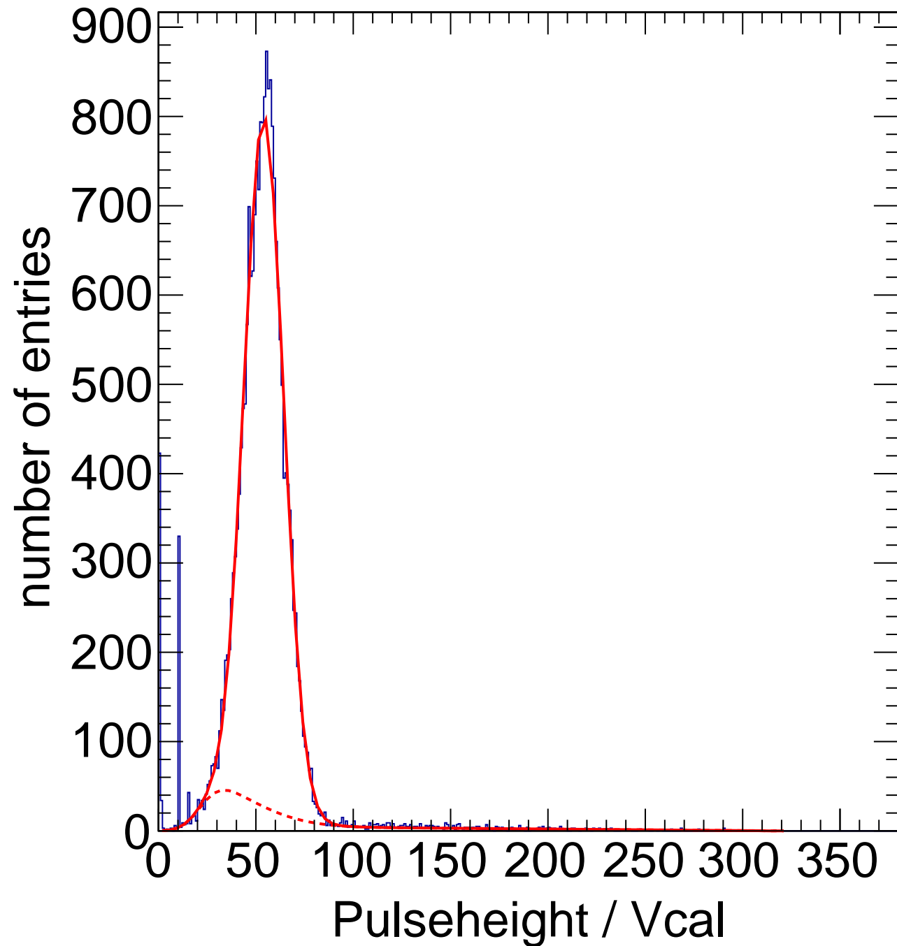
X-ray Calibration - Target Zn Method Spectrum Chip C15
