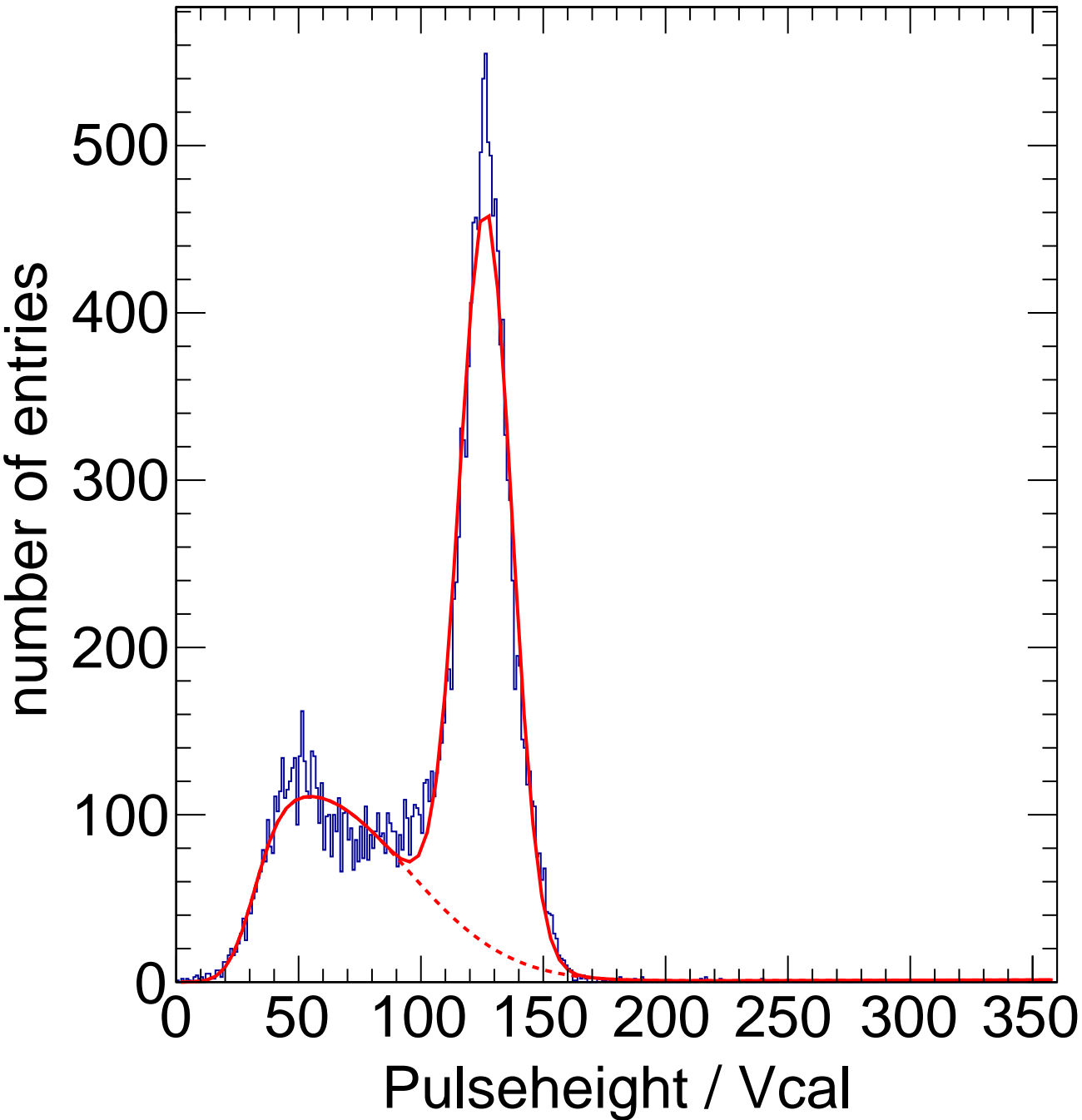
X-ray Calibration - Target Ag Method Spectrum Chip C1
