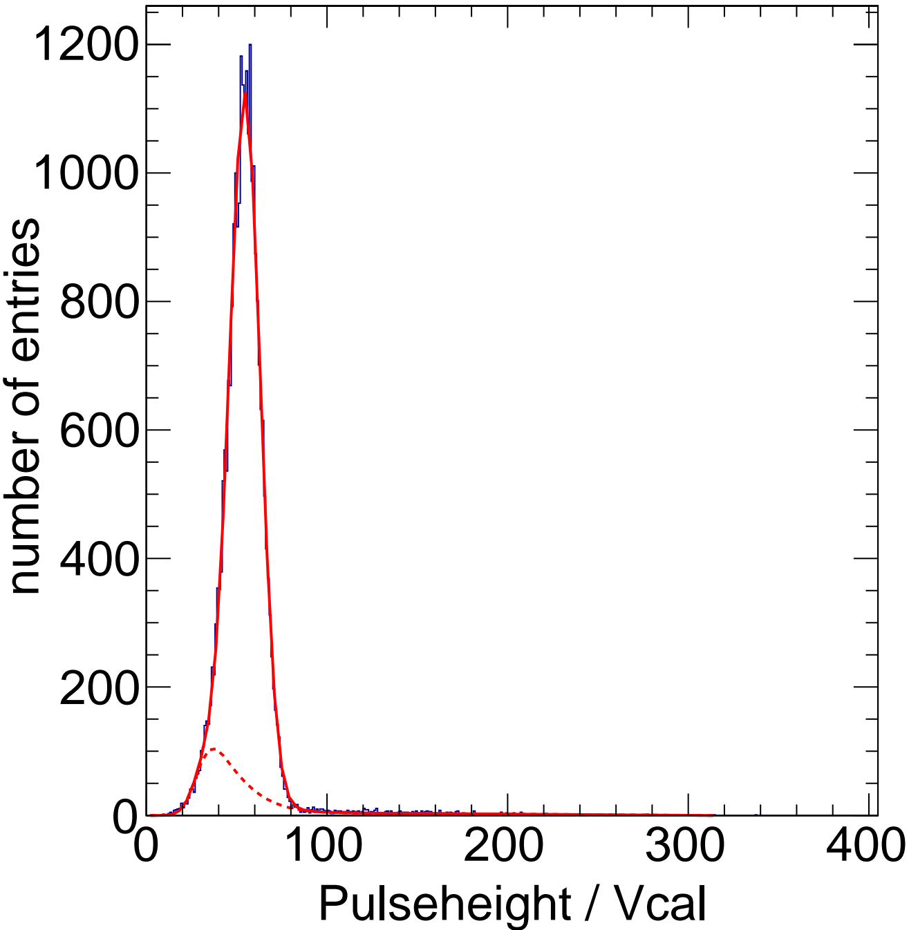
X-ray Calibration - Target Zn Method Spectrum Chip C8
