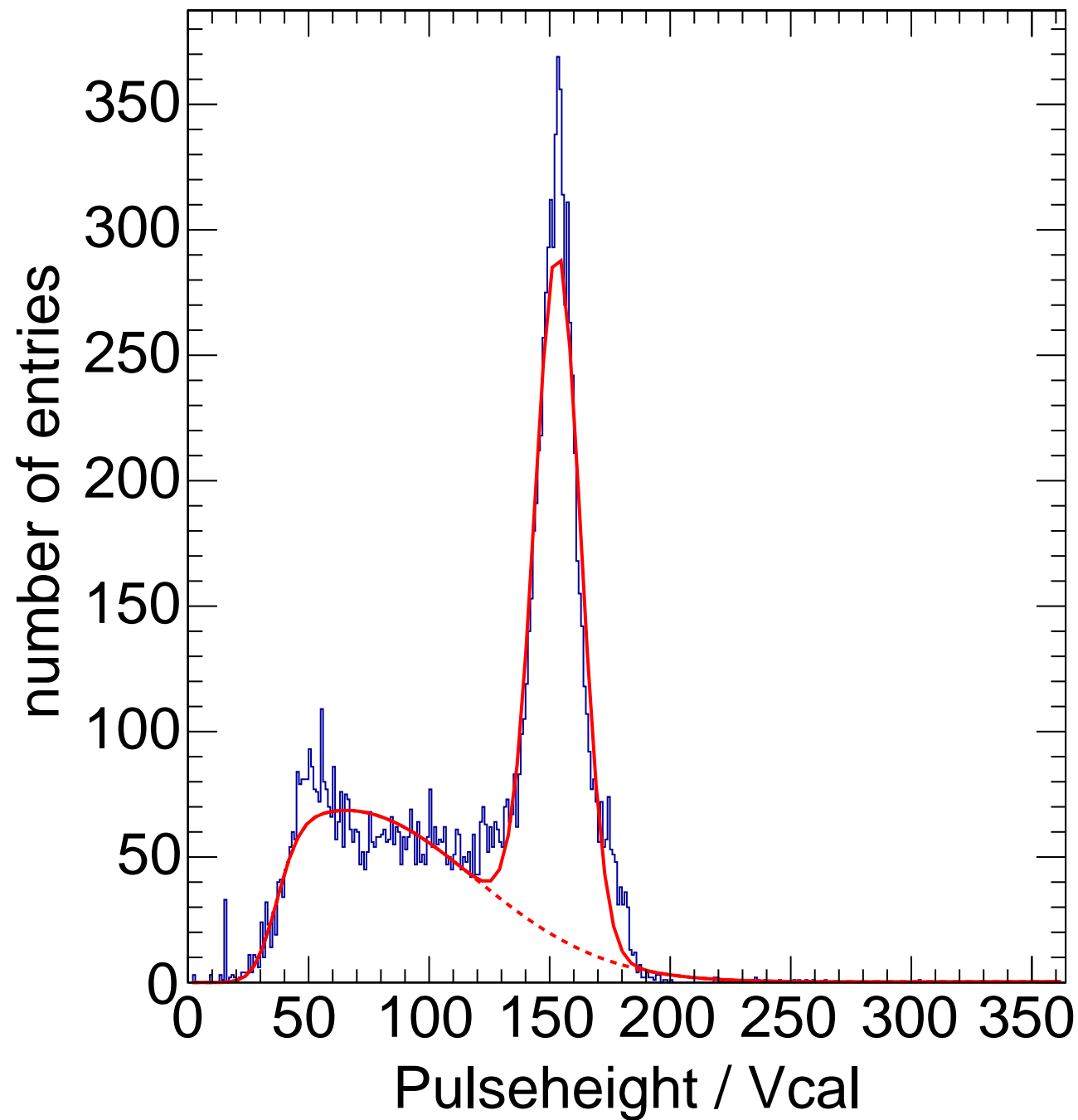
X-ray Calibration - Target Sn Method Spectrum Chip C9
