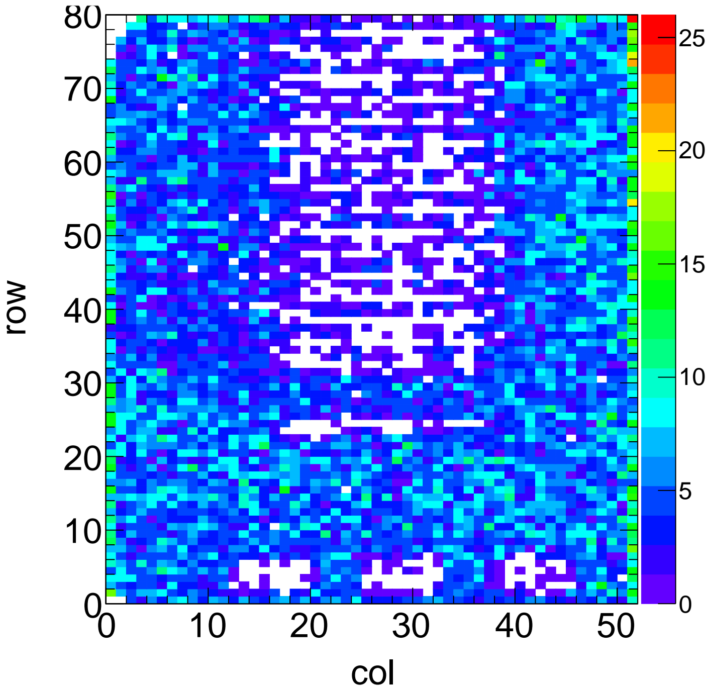
X-ray Hit Map - Target Ag Method Spectrum Chip C2
