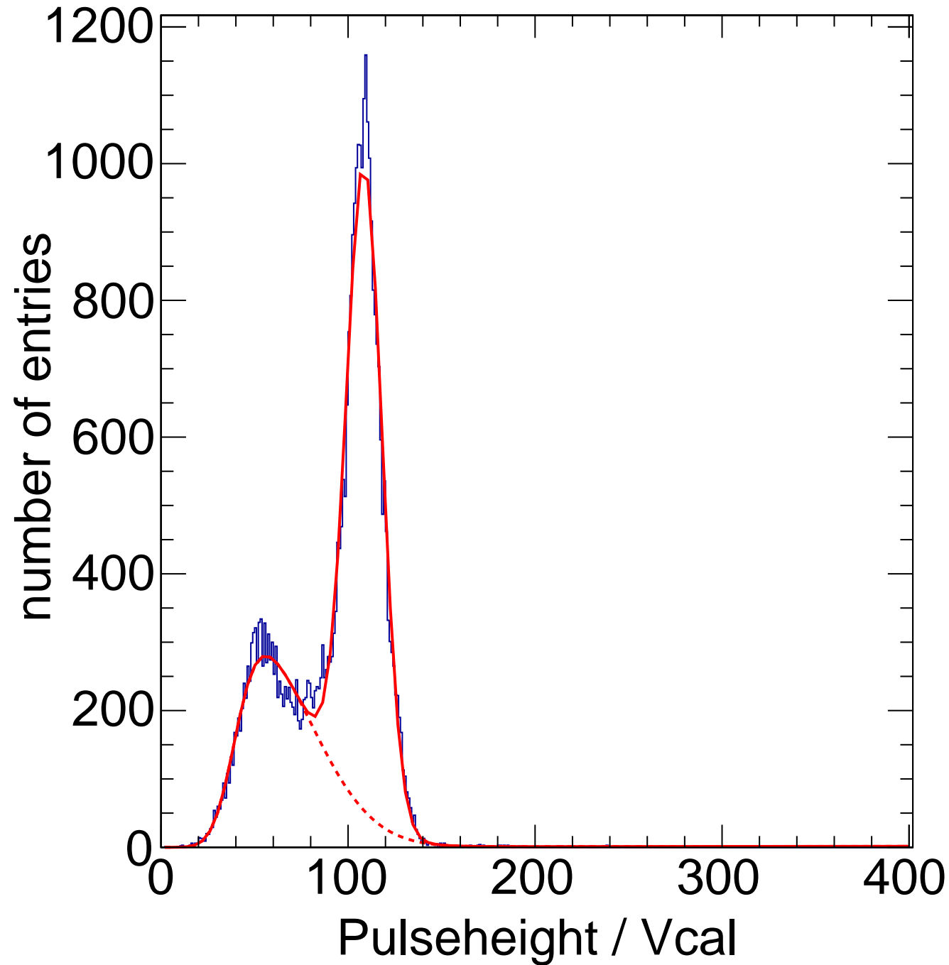
X-ray Calibration - Target Mo Method Spectrum Chip C15
