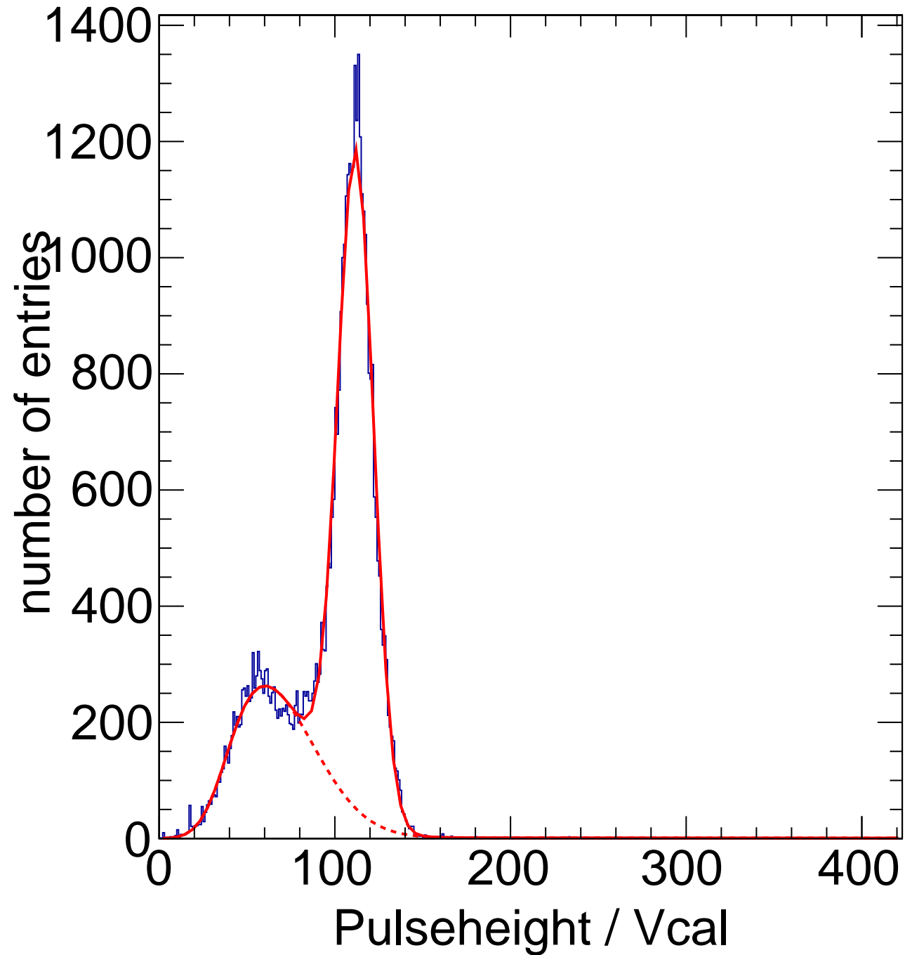
X-ray Calibration - Target Mo Method Spectrum Chip C10
