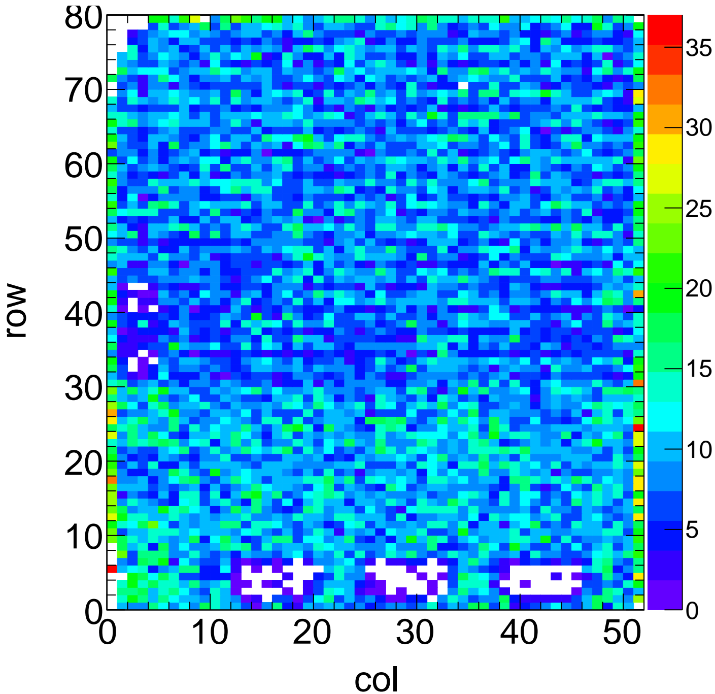
X-ray Hit Map - Target Mo Method Spectrum Chip C0
