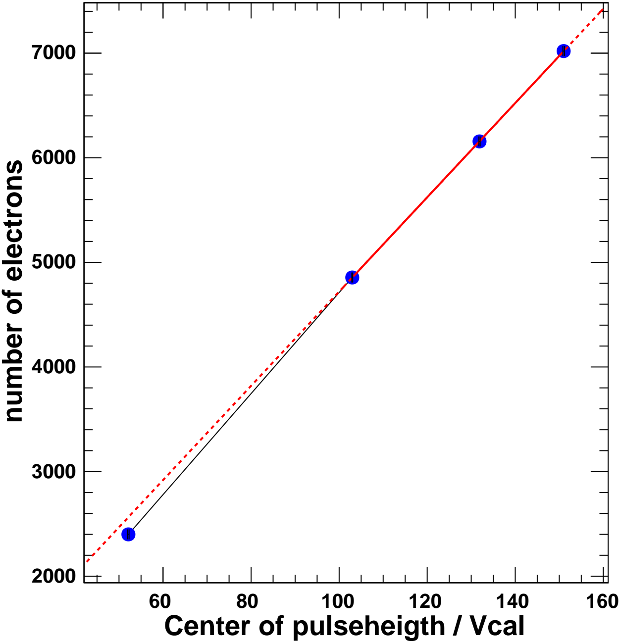
X-ray Calibration - Vcal Calibration Method Spectrum Chip C2
