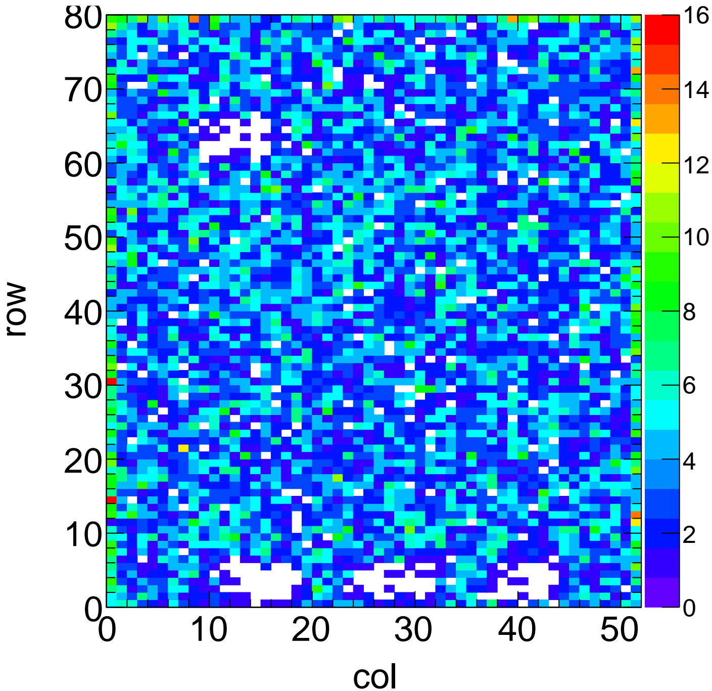
X-ray Hit Map - Target Sn Method Spectrum Chip C3
