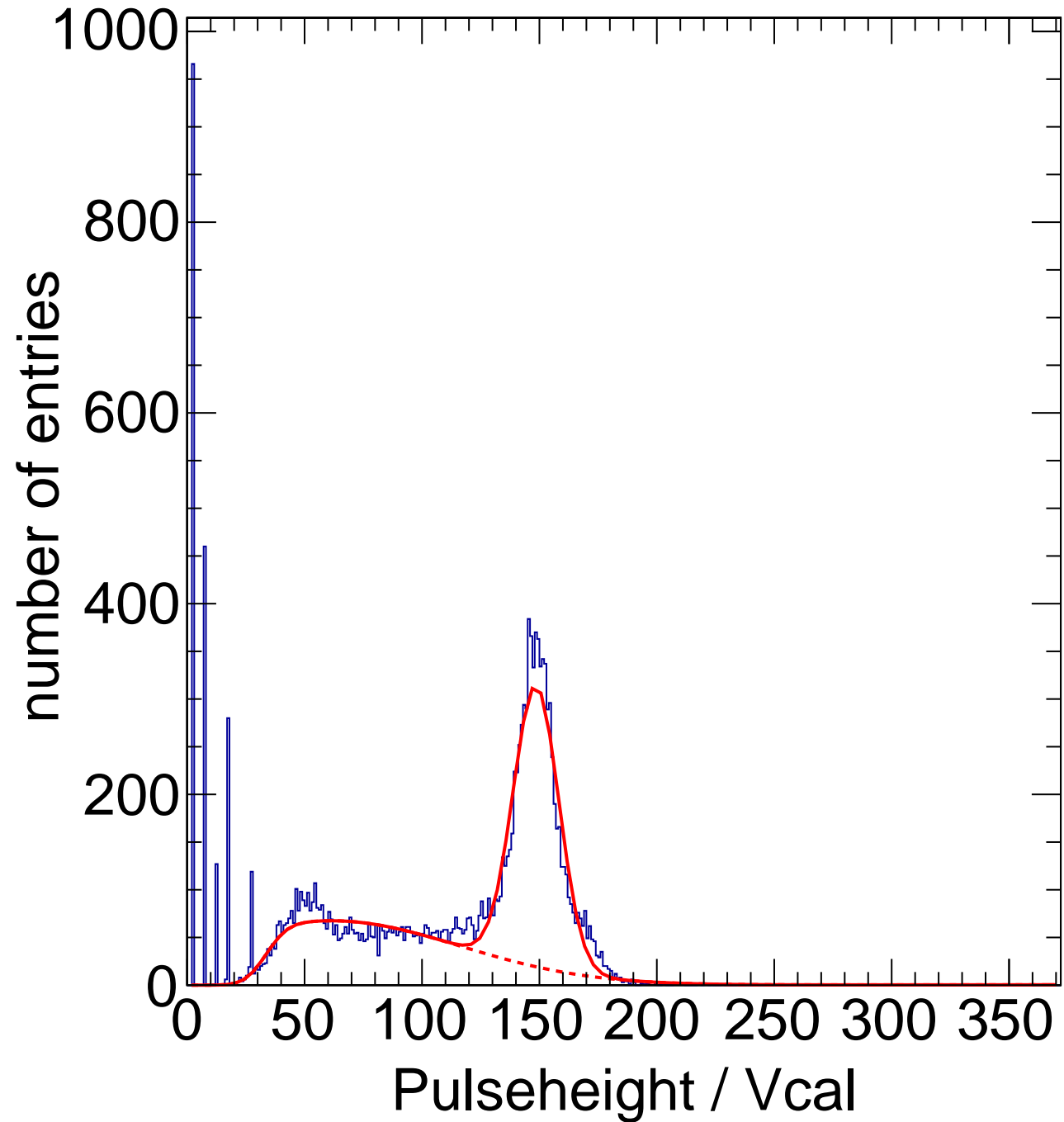
X-ray Calibration - Target Sn Method Spectrum Chip C8
