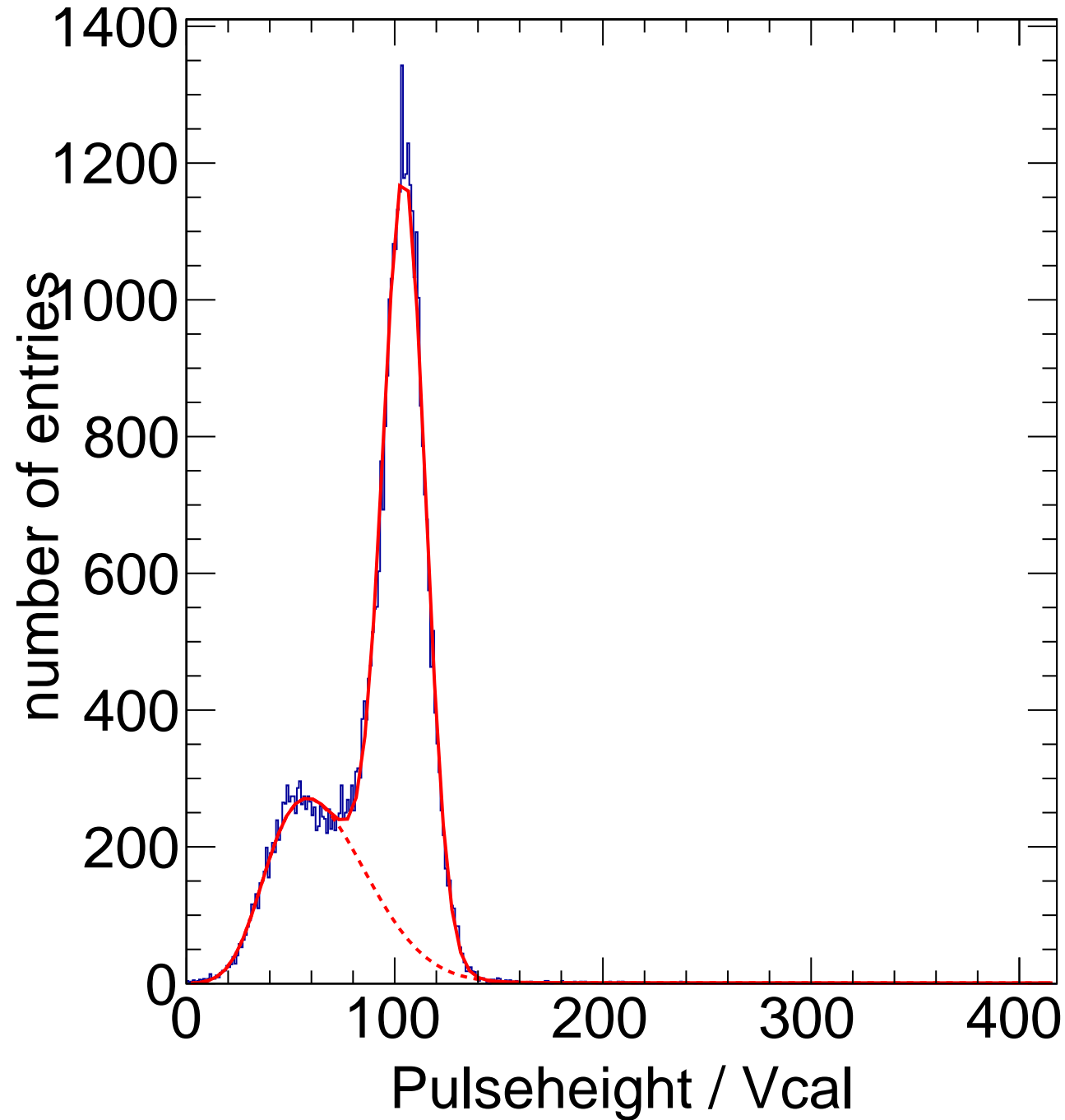
X-ray Calibration - Target Mo Method Spectrum Chip C5
