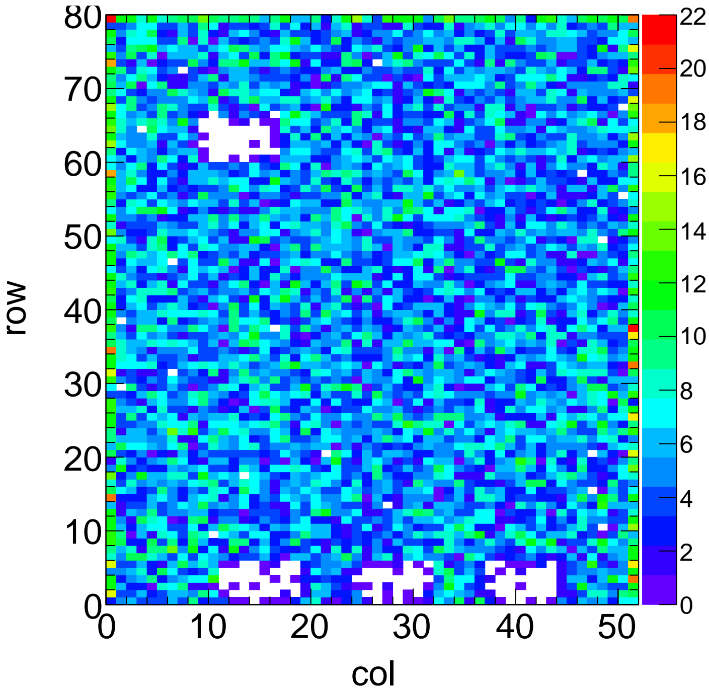
X-ray Hit Map - Target Ag Method Spectrum Chip C3
