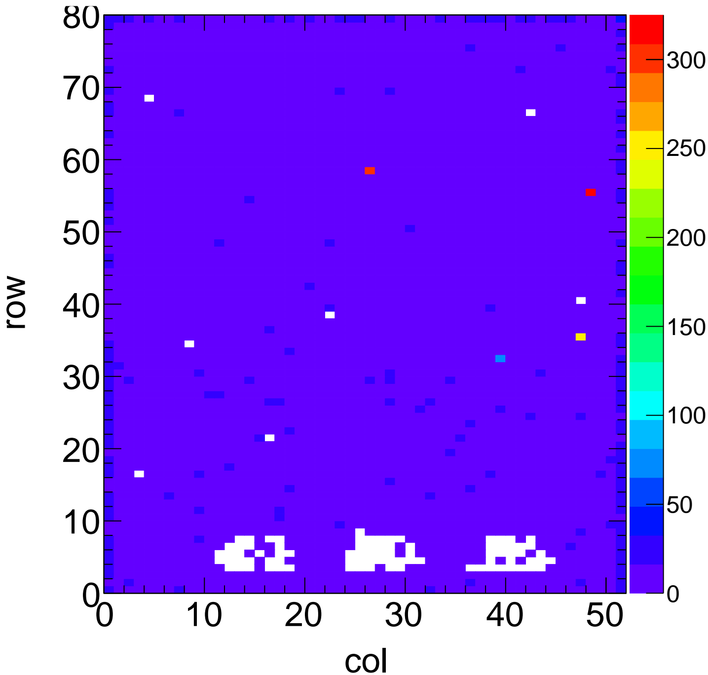
X-ray Hit Map - Target Mo Method Spectrum Chip C14
